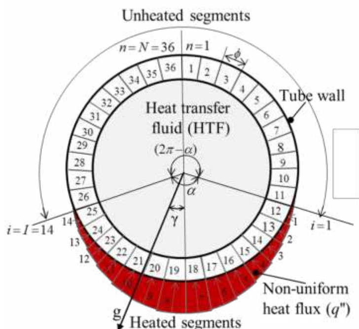
Figure 3 Cross-section of Figure 2 with sinusoidal non-uniform heat flux distributions and gravity ( g ) directed at angle \gamma
