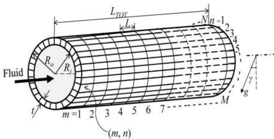
Figure 2 Tube model divided into M \times N numerical surfaces
