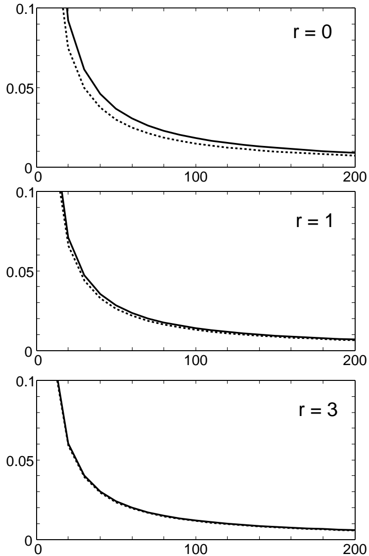
Figure 2: Theoretical learning curves of the Fisher kernel classifier. The horizontal axis shows the number of labeled samples n and the vertical axis shows the generalization error \mathbb{E}[R(\hat{\eta})] . The solid and broken curves correspond to the generalization error of the two step estimator and the lowerbound determined by the Cramér-Rao bound, respectively. As the unlabeled/labeled ratio r increases, the two curves get closer.
