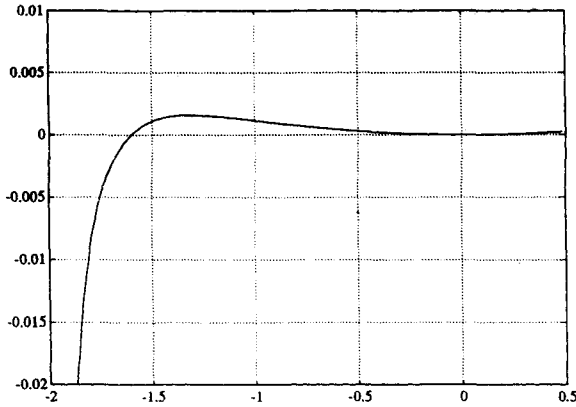
Fig. 3. D(\lambda) vs. \lambda for p = 3, c = 3
