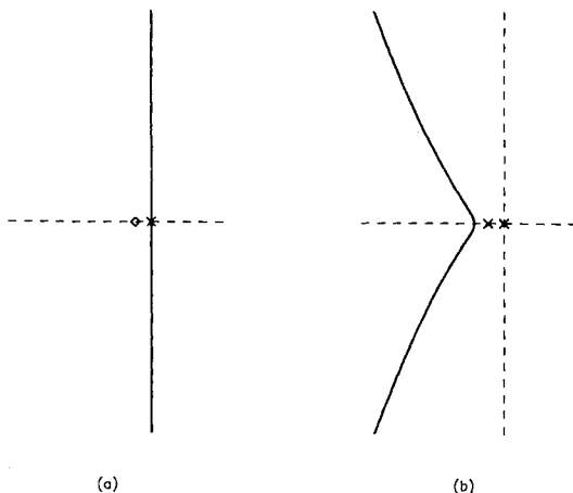
Fig. 2. (a) Spectrum of \partial_y L_c for p near 4. ‘◊’ marks resonance pole. (b) Spectrum of A_a . ‘×’s mark eigenvalues
