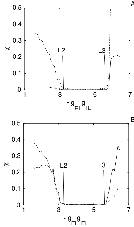
Figure 19: The synchrony level of the excitatory (solid line) and the inhibitory populations (dashed line) vs. -g_{EI}g_{IE} . The strength of the E-E and I-I interactions is fixed: g_{EE} = 2 , g_{II} = -2 . Other parameters \nu_E = \nu_I = 50 Hz, \sigma_E = \sigma_I = 0.1 . A network with N_E = N_I = 1600 neurons was simulated for different values of g_{EI} and a fixed ratio g_{EI}/g_{IE} . (A) g_{EI}/g_{IE} = -1/4 (B) g_{EI}/g_{IE} = -4 . The level of synchrony of the two populations was calculated as explained in appendix C (average over 6 seconds). The theory predicts that the AS becomes unstable at -g_{EI}g_{IE} = 2.96 (on L2) and -g_{EI}g_{IE} = 5.42 (on L3) as indicated by the arrows.
