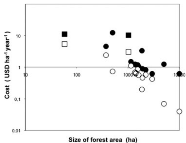
Figure 2 Comparison of the cost of monitoring the condition of forests by local people and trained scientists. Cost of measurements of woody biomass by community members (□) and professional experts (■) and of cut trees by community members (○) and professional experts (●) (log 10 scales).
