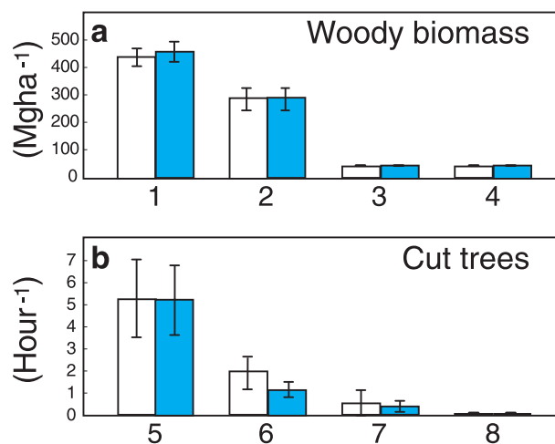
Figure 1 Comparison of forest condition data compiled by local people and trained scientists. Measurements of woody biomass (a, core sites 1–4) and cut trees (b, core sites 5–8) ( \pm S.E.) by community members (white) and professional experts (blue) over a range of forest biomass and resource use intensities in dense oak forest (core site 1), oak forest (core site 2), and degraded forest (core site 3) in India, miombo woodland in Tanzania (core sites 4–6), and dry deciduous forest in Madagascar (core sites 7–8). Data from the other 11 study sites are provided in Table 2.
