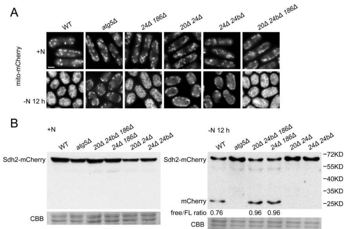
Fig. 4. Mitochondrial autophagy is promoted in a redundant manner by Atg20, Atg24 and Atg24b. (A) Starvation-induced vacuole localization of mito-mCherry was monitored in selected double and triple mutants. 20, Atg20; 24, Atg24; 24b, Atg24b; 186, Mug186. +N, nitrogen-containing medium; –N, nitrogen-starvation medium. Scale bar: 3 \mu m. (B) Starvation-induced processing of Sdh2–mCherry was monitored in selected double and triple mutants. Coomassie Brilliant Blue R-350 (CBB) staining of PVDF membrane after immunodetection was used to control for protein loading and blotting efficiency. The free/FL ratios were calculated as described in Fig. 1.
