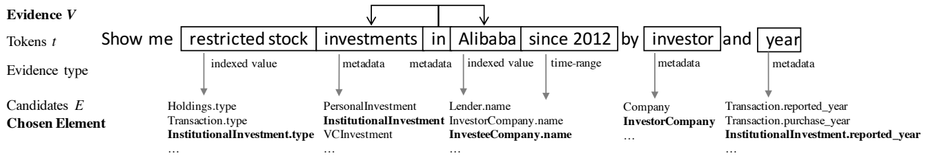
Figure 3: A Natural Language Query annotated with the Evidence Set V obtained from the Ontology Evidence Annotator.
