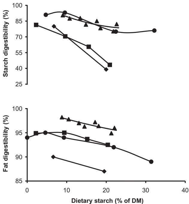
Fig. 6.1. Apparent digestibility of starch and fat in salmon fed diets with different dietary starch concentrations. ■, Aksnes (1995), 0.6 kg salmon in salt water; ●, Hemre et al. (1995a), 80 g post-smolt in brackish water (20 g l -1 ); ▲, Grisdale-Helland and Helland (1997), 80 g fingerlings in fresh water; ◆, Krogdahl et al. (1999), 1.9 kg salmon in salt water; DM, dry matter.
