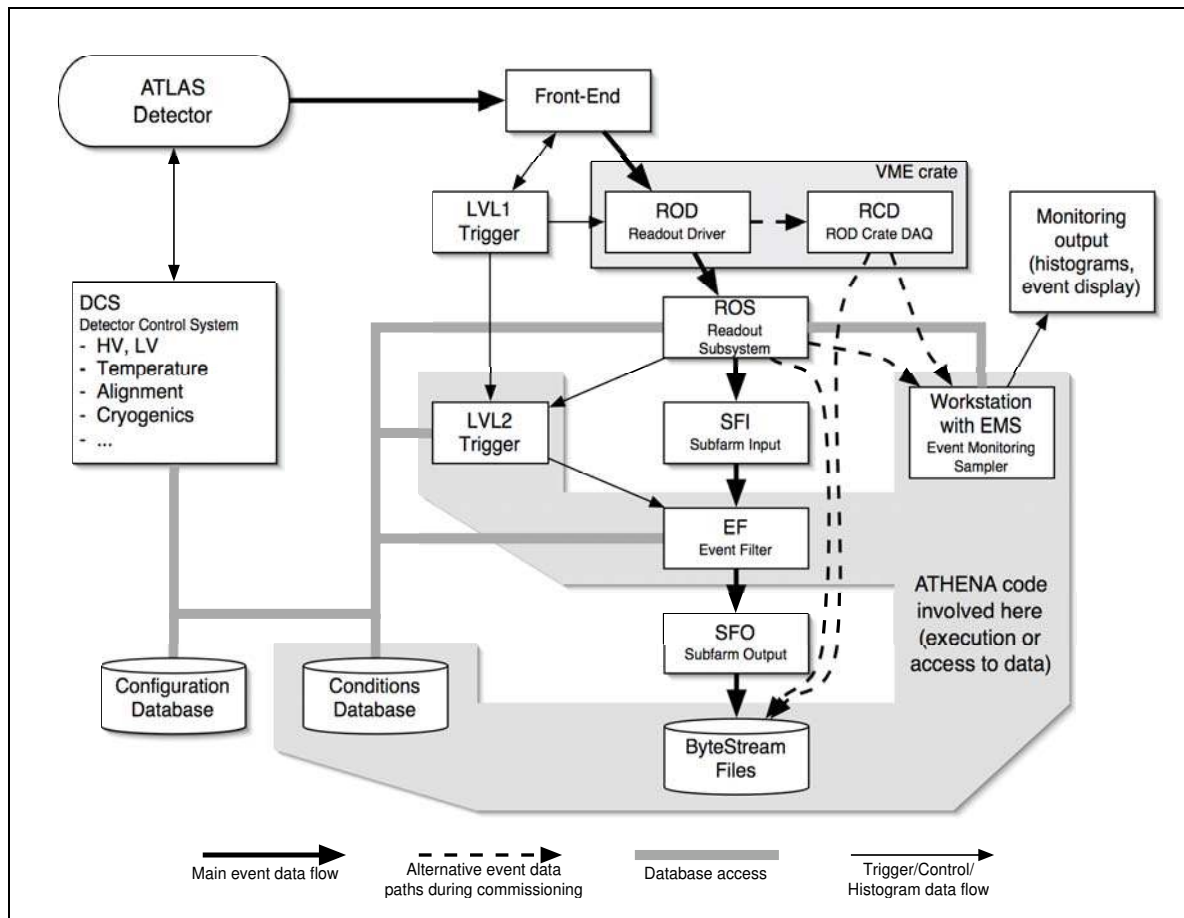
Figure 3-14 Data flow of events and conditions data.
