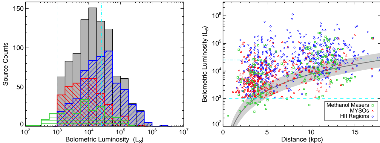
Figure 19. Left panel: The bolometric luminosity distribution of all matched RMS sources is shown in grey while that of the methanol-maser, MYSO and H II-region samples are shown in green, red and blue, respectively. The dashed and dash-dot vertical cyan lines indicate the luminosity cut applied to the RMS sample to insure only massive star-forming clumps are selected (i.e., L_{\text{bol}} > 1000 L_{\odot} ) and the RMS completeness limit at \sim 20 kpc, respectively. The bin size is 0.25 dex. Right panel: The luminosity distribution as a function of heliocentric distance. The dark line and light grey shaded region indicate the limiting sensitivity of the MSX 21- \mu\text{m} band and its associated uncertainty. The horizontal cyan lines are the same as described for the left panel. Where multiple sources have been identified within the MSX beam, the luminosity has been apportioned between them resulting in some sources being located below the sensitivity limit (see Mottram et al. 2011b for details).
