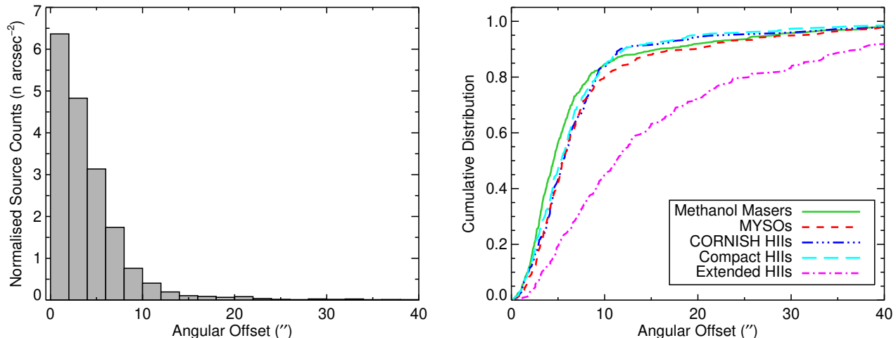
Figure 2. Left panel: Normalised source counts for the ATLASGAL-RMS matches are shown as a function of offset between their position and that of the peak of the submillimetre emission of their associated ATLASGAL source. We have truncated the x-axis of this plot at 40'' as there are only 34 matches that have a larger angular separation ( \leq 80'' ) and the surface density effectively falls to zero. The bin size is 2''. Right panel: Cumulative distribution of angular offset of the methanol masers, MYSOs and H II regions drawn from the MMB, AMGPS, CORNISH and RMS surveys.
