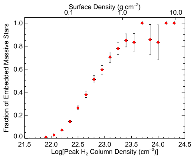
Figure 13. Fraction of massive star forming clumps as a function of peak column density. The bin size is 0.15 dex and the uncertainties are estimated using binomial statistics.
