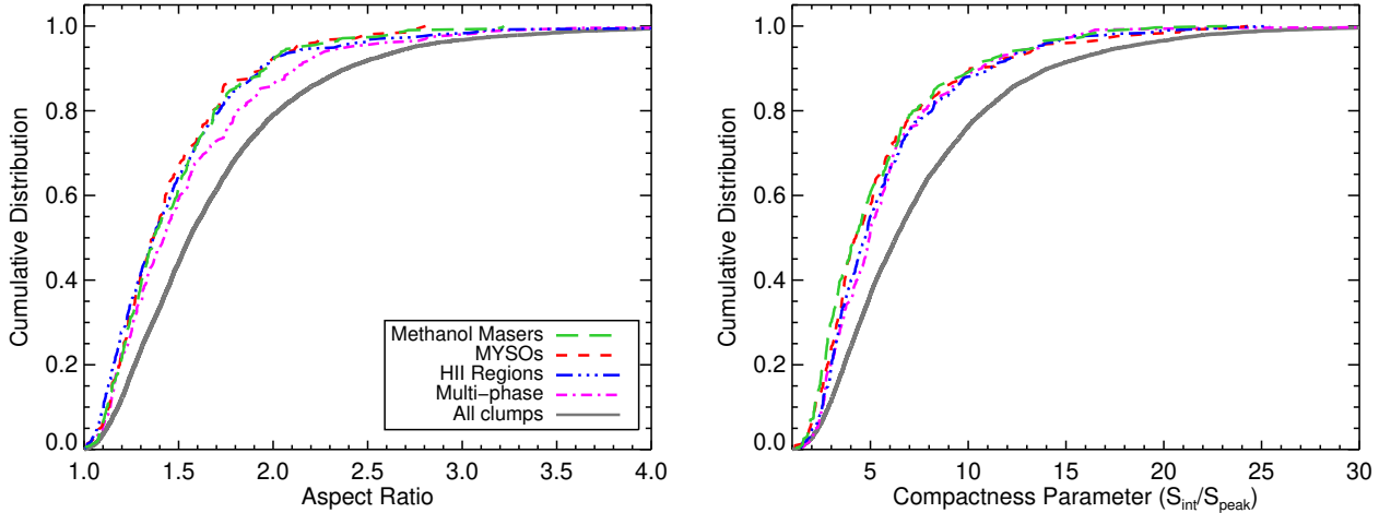
Figure 4. The cumulative distributions of the aspect ratio and compactness parameter (Y-factor) are presented in the left and right panels, respectively. In these plots we show the distributions of the four subsamples of MSF clumps and the unassociated clumps separately (see legend left panel for colours and line styles for both plots).
