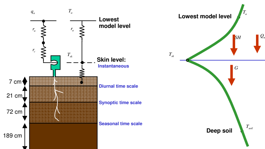
Figure 1 Illustration of the 4-layer land surface model (left; Viterbo and Beljaars 1995) and a schematic temperature profile in soil and lower atmosphere in surface cooling conditions (right).
