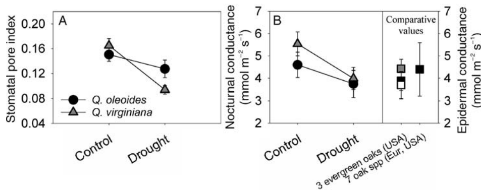
Figure 6. A: Stomatal pore index for the well-watered control and drought-treated Q. oleoides and Q. virginiana sapling leaves. B: Nocturnal conductance, calculated for a two sided leaf, compared to epidermal conductance for three evergreen oak species measured on detached leaves in a separate study (Cavender-Bares 2000) and to the mean value of epidermal conductance for 7 European and American oaks (Kerstiens et al. 1996). Symbols: Q. oleoides (●); Q. virginiana (▲); Q. myrtifolia (□); Q. virginiana (■) and Q. geminata (■). Error bars are \pm SE.
