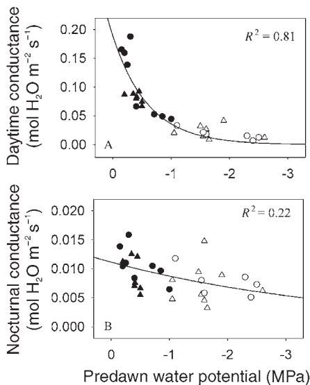
Figure 4. Daytime conductance (A) and nocturnal conductance (B) decrease exponentially with decreasing predawn water potential. Note the difference in scale on the y-axes of the two graphs. Open symbols correspond to plants in the drought treatment and closed symbols to the well-watered treatment for the two live oak species Q. virginiana (○, ●) and Q. oleoides (△, ▲).
