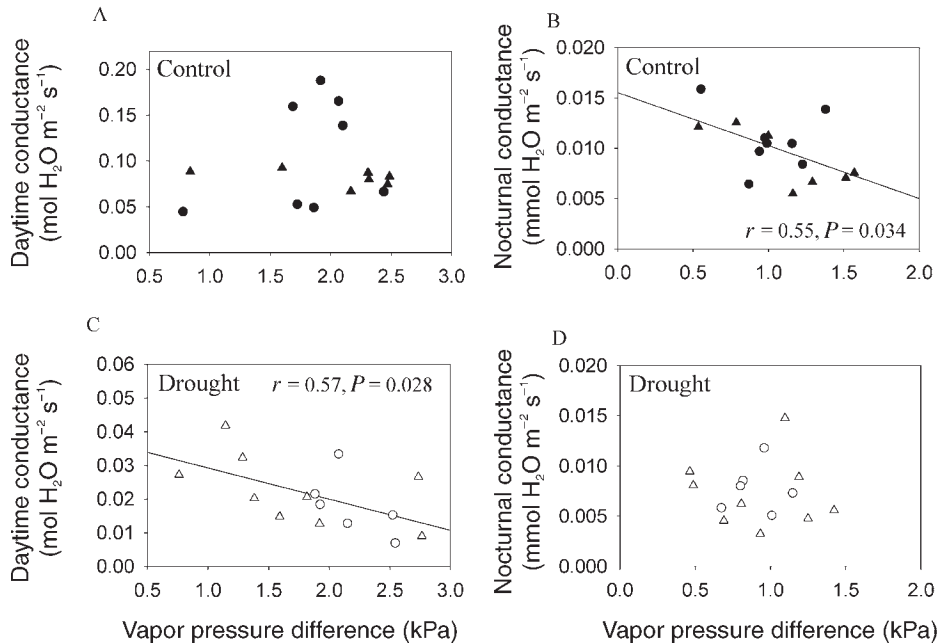
Figure 3. Nocturnal conductance decreases with increasing leaf-to-air vapor pressure difference in well-watered (control) plants (B), but there is no relationship in drought-treated plants (D). Daytime conductance does not vary with vapor pressure difference in well-watered (control) plants (A), but in drought-treated plants daytime conductance decreases with increasing leaf-to-air vapor pressure difference (C). Open symbols correspond to plants in the drought treatment and closed symbols to plants in the well-watered treatment for the live oak species Q. virginiana (○, ●) and Q. oleoides (△, ▲).
