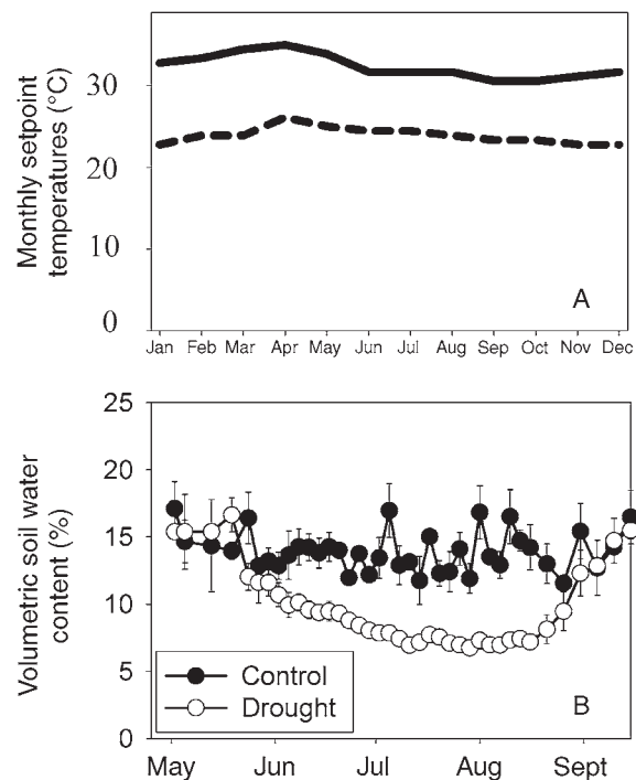
Figure 1. A: Monthly maximum and minimum temperature setpoints. B: A drought treatment was imposed from May–August, corresponding with the drought season in northwest Costa Rica. The volumetric soil water content of the control (●) and drought-treated (○) pots is shown for May–September 2005. Error bars are \pm SE, n=24 per treatment.
