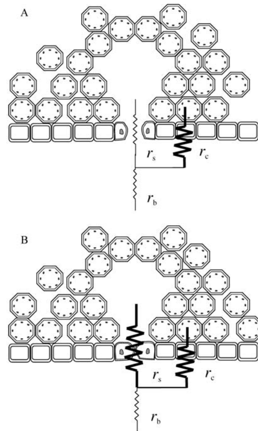
Figure 7. Schematic of resistances (reciprocal of conductance) to the diffusion of water vapor across the leaf surface when stomata are open (A) and closed (B) (adapted from Pearcy et al. 1989). Cuticular resistance ( r_c ) and stomatal resistance ( r_s ) are in parallel with each other and in series with boundary layer resistance ( r_b ). When stomata are open, stomatal and boundary layer resistances are much lower than cuticular resistance. When stomata are closed, both stomatal and cuticular resistances are high, making boundary layer resistance inconsequential.
