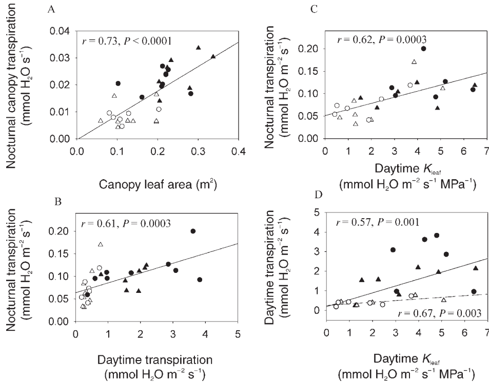
Figure 5. Correlates of nocturnal transpiration. Nocturnal whole canopy water loss is correlated with total canopy leaf area (A); nocturnal transpiration rate per leaf area is correlated with daytime transpiration rate (B), and with leaf hydraulic conductance ( K_{leaf} ) (C). For comparison, the relationship between daytime transpiration and K_{leaf} is shown (D). While there is a significant relationship, the daytime conductance values for the drought-treated plants show a tighter correspondence with K_{leaf} (dashed line) than the combined data (solid line). Daytime transpiration rates of the well-watered plants alone are not significantly correlated with K_{leaf} . Open symbols represent drought-treated plants and closed symbols represent well-watered plants of the live oak species Q. virginiana (○,●) and Q. oleoides (△,▲).
