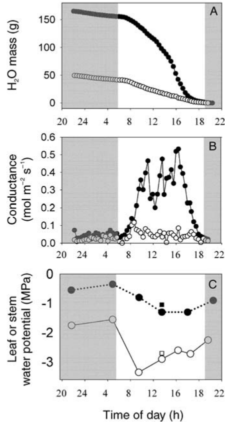
Figure 2. Representative examples of the diel course of transpirational water loss (A), total conductance to water vapor per unit leaf area (B) and leaf or stem water potential (C) for a drought-treated (open symbols) and well-watered (closed symbols) plant. Symbols: leaf (○, ●); and stem (□, ■).
