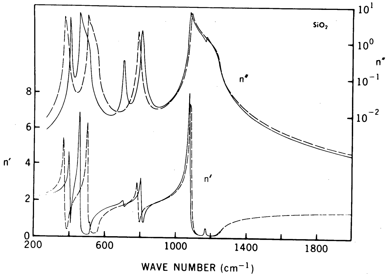
Figure 10. Complex refractive indices of SiO 2 in the infrared. The real part of the refractive index is indicated by n' and the imaginary part by n'' . Indices for the ordinary ray are represented by solid lines and for the extraordinary rays by dashed lines.
