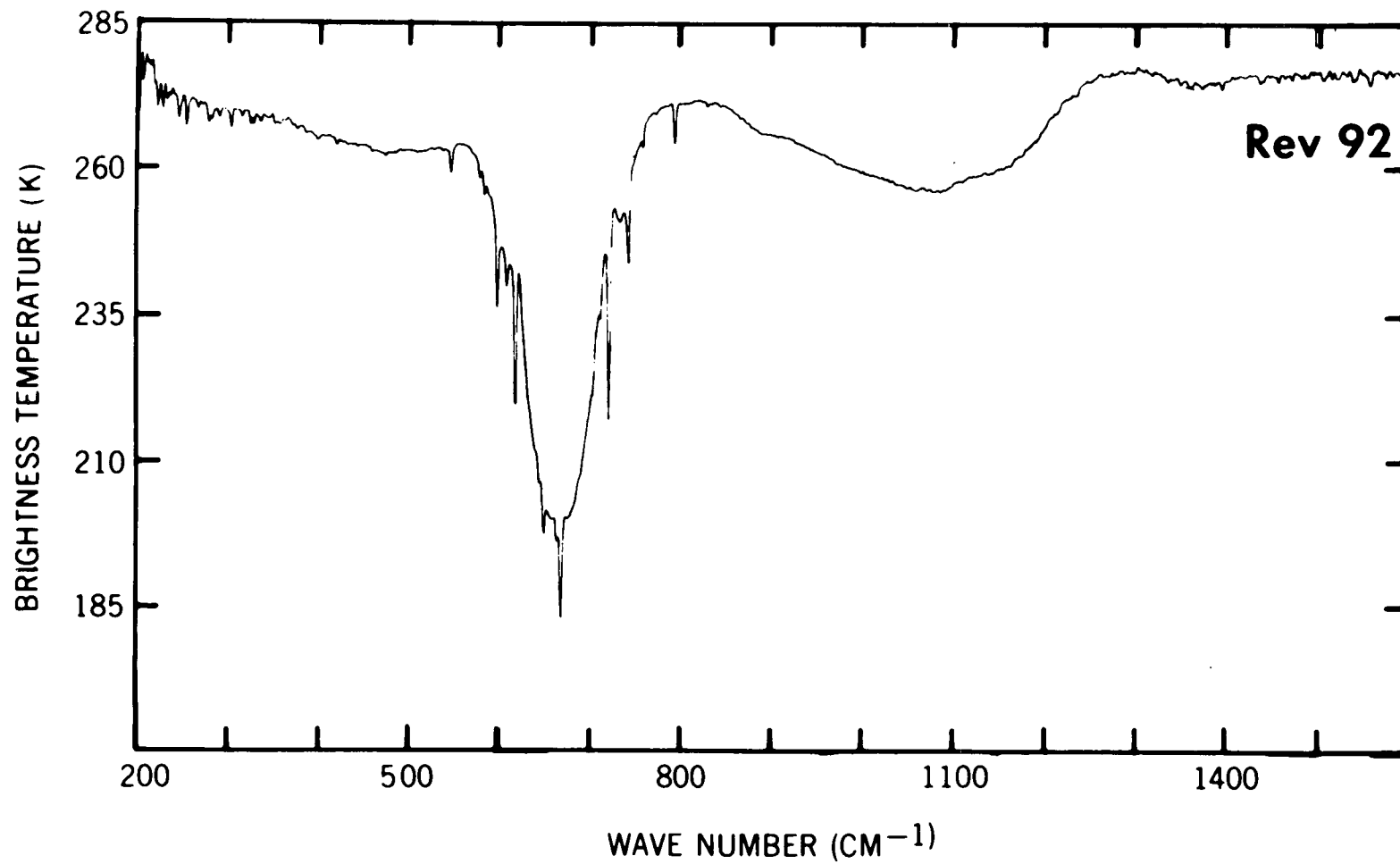
Figure 14. Measured brightness temperature spectrum from revolution 92 showing diffuse spectral features due to atmospheric dust.
