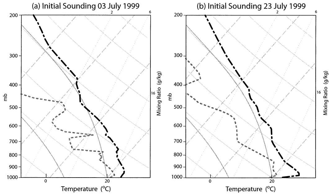
FIG. 2. Profile of initial conditions for (a) 3 Jul 1999: CTP = 87 \text{ J kg}^{-1} , HI_{low} = 10.6^\circ\text{C} , rainfall occurs only over wet soils; and (b) 23 Jul 1999: CTP = 254 \text{ J kg}^{-1} , HI_{low} = 11.6^\circ\text{C} , rainfall occurs only over dry soils. Thick dashed-dotted line is profile temperature; thick dashed line is profile dewpoint temperature; light solid lines are dry adiabats; long-dashed lines are constant temperature; dotted lines are constant mixing ratio.
