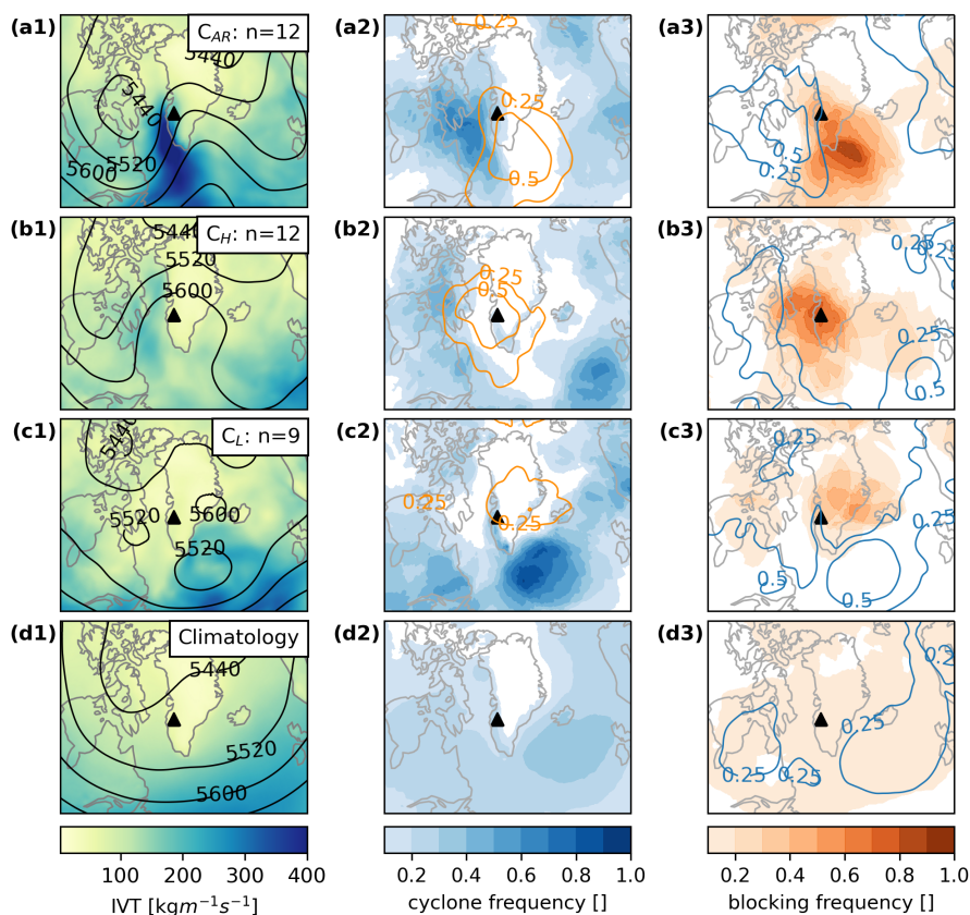
Figure 7. Left column (a1, b1, c1, and d1): Composites of IVT (colorbar) and Z500 (black contours) of all MI-days per cluster, as well as for the climatology (average over all days from May to October 2009–2012). Middle column (a2, b2, c2, and d2): Same as the left column but for composites of cyclone frequency (shaded blue) and blocking frequency (orange contours), calculated as explained in Sec. 2.4. Right column (a3, b3, c3, and d3): Same as the left column but for composites of the blocking frequency (shaded orange) and cyclone frequency (blue contours). The location of the Russell Glacier is indicated with a black triangle.
