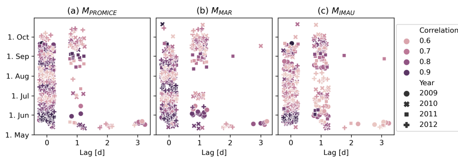
Figure 4. DOY versus the time lag in the cross-correlation between V_{ice} and melt data from a) M_{PROMICE} , b) M_{MAR} , c) M_{IMAU} , calculated for 20-day moving windows in May–October for 2009–2012. DOY values in the figure mark the centre of each 20-day window. Only values with a cross-correlation coefficient larger than 0.5 are plotted for each lag in time. The color of the points refers to the correlation value, while the marker of the points indicates the year.
