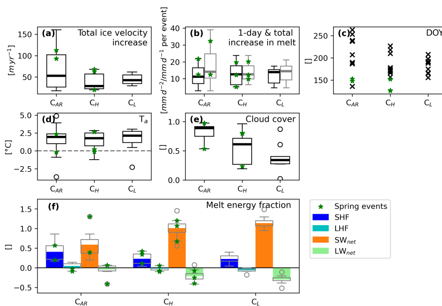
Figure 9. Boxplots for each of the three main clusters ( C_{AR} , C_H and C_L ) for the MI-days showing composites of (a) total ice velocity increase, (b) 1-day (black) and total melt-increase (grey) for each melt-induced speed-up, and (c) day-of-year, DOY (d) air temperature ( T_a ), (e) cloud cover, and (f) melt energy fraction of different components of SEB - sensible heat flux (SHF), latent heat flux (LHF), net shortwave radiation ( SW_{net} ) and net longwave radiation ( LW_{net} ). Melt-increase data represents an average over the three melt datasets, only during days where the increase is consistent among them (Sec. 3.3). Spring events are marked with green stars in each panel.
