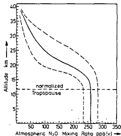
Fig. 2. Mean vertical distribution of atmospheric N_2O . Dashed lines indicate the scatter of data.
