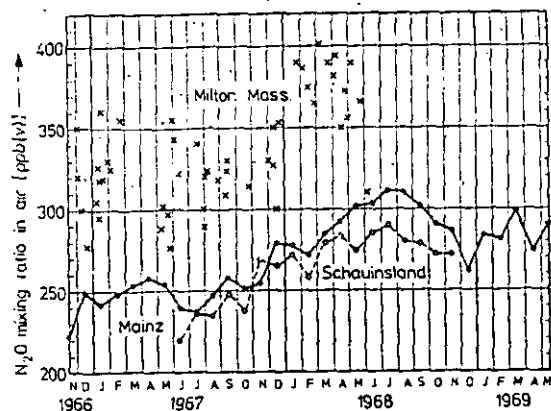
Fig. 1. Long-term fluctuations of tropospheric N_2O as measured in Mainz and Schauinsland (W.-Germany) and in Milton (Mass., USA). Crosses denote individual measurements, circles denote monthly average values.
