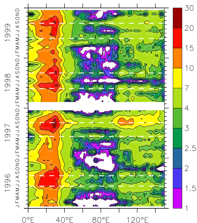
Fig. 51. Tropospheric \text{NO}_2 column (in 10^{14} molecules/ \text{cm}^2 ) averaged for 5^\circ\text{N} – 30^\circ\text{S} during 1996–1999 from the GOME satellite instrument (from Kunhikrishnan et al., 2004, copyright 2004 by the American Geophysical Union, reproduced with permission).
