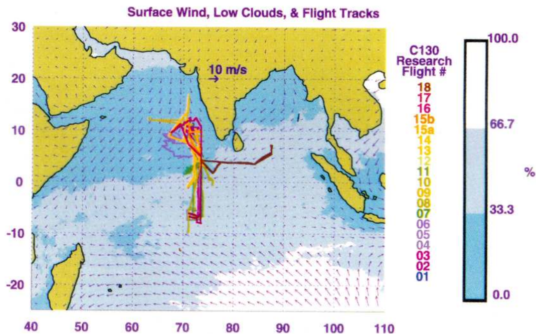
Fig. 12. Flight tracks of the NCAR C-130 during the INDOEX intensive field phase (IFP), overlaid on the mean surface wind data from the NCEP/NCAR reanalysis (from Ramanathan et al., 2001, copyright 2001 by the American Geophysical Union, reproduced with permission).
