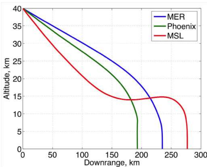
Figure 1 - Comparison of entry trajectory downrange versus altitude for MER, Phoenix, and MSL
