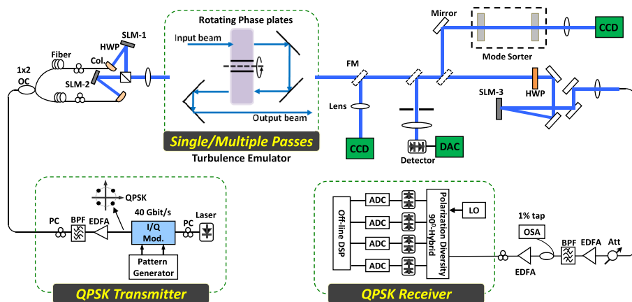
Fig. 2. Experimental setup of an OAM multiplexed FSO communication system. BPF, bandpass filter; Col., Collimator; EDFA, erbium-doped fiber amplifier; FM, flip mirror; DAC, digital–analog converter; DSP, digital signal processing; HWP, half-wave plate; LO, local oscillator; OC, optical coupler; QPSK, quadrature phase shift keying.
