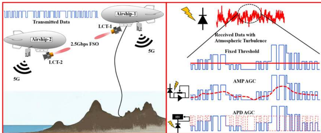
Fig. 1. Schematic diagram of the 5G floating base station and laser link (left), the mechanism and suppression measures of atmospheric turbulence flicker on the communication receiver (right).
