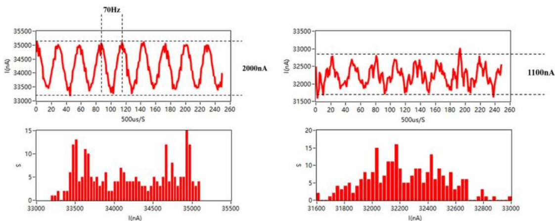
Fig. 6. Output signal of fixed gain (left) and adaptive gain (right) under the action of 70 Hz sinusoidal light intensity signal.
