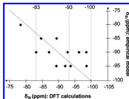
Figure 4. Comparison of ^{29}\text{Si} chemical shifts calculated by DFT and an empirical model (see Figure S18), derived from the analysis of the literature data available, assuming 2-fold coordination for all O atoms, and constant chemical shift variation by +10 ppm for each ^1\text{H} and +5 ppm for each Al second neighbor. 85–89 The experimental ^{29}\text{Si} chemical shifts of our Si/ \text{Al}_2\text{O}_3 samples are represented with the dotted vertical lines. The plain line depicts the diagonal of the parity plot.
