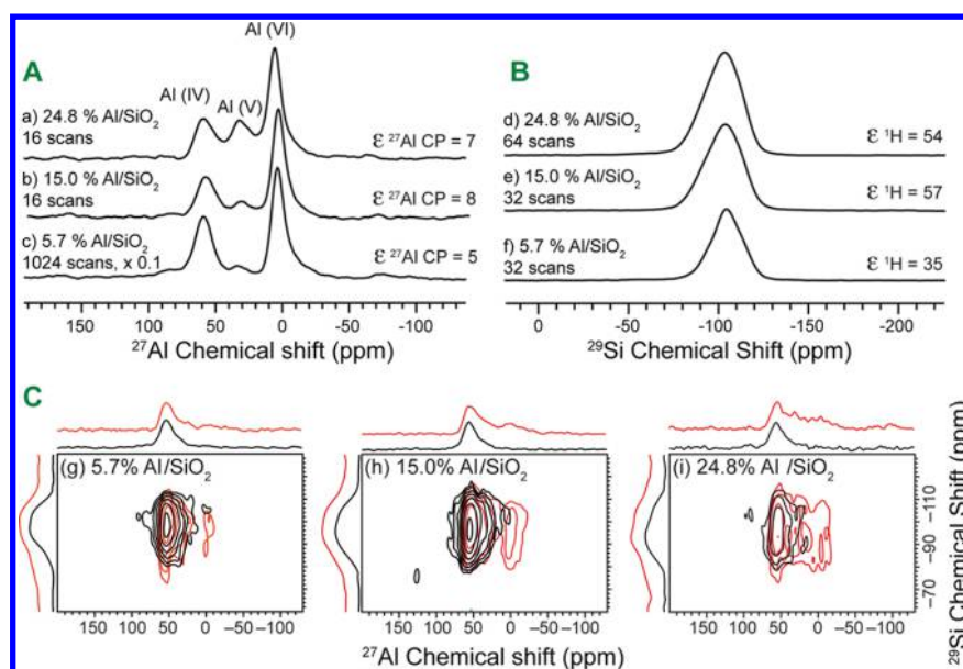
Figure 1. (A) DNP enhanced 1 H- 27 Al CPMAS solid-state NMR spectra acquired at 600 MHz/395 GHz: (a) 24.8 wt % Al/SiO 2 , (b) 15.0 wt % Al/SiO 2 , (c) 5.7 wt % Al/SiO 2 . Spectra for all of these samples were also measured on a 400 MHz DNP spectrometer (Figure S3, ESI). The recycle delay was 3.5 s. (B) DNP SENS (400 MHz/263 GHz) 1 H- 29 Si CPMAS solid-state NMR spectra: (d) 24.8 wt % Al/SiO 2 , (e) 15.0 wt % Al/SiO 2 , (f) 5.7 wt % Al/SiO 2 . For 29 Si measurement, DNP enhancement was measured by directly observing the 1 H spectrum, since the acquisition of a 29 Si CPMAS spectrum without DNP required too long for signal averaging. All spectra were acquired with a 12.5 kHz spinning frequency and a CP contact time of 0.6 ms for 27 Al and 3.0 ms for 29 Si. 1 H- 29 Si CPMAS spectrum of the starting silica is available Figure S7. (C) DNP SENS (400 MHz/263 GHz) scalar refocused INEPT (black traces/contours) and dipolar refocused R 3 -INEPT (red traces/contours) 29 Si- 27 Al heteronuclear correlation spectra: (g) 5.7 wt % Al/SiO 2 , (h) 15.0 wt % Al/SiO 2 , (i) 24.8 wt % Al/SiO 2 . All spectra were acquired with a 12.5 kHz MAS frequency. Projections of the 2D spectra are shown along the horizontal and vertical axes. For dipolar correlation experiments, 96 total rotor cycles ( N , Figure S1) of recoupling were used, while for scalar correlation experiments, 420 total rotor cycles of evolution were used. Spectra were acquired with between 16 and 80 scans per increment, 28 t 1 increments, and a rotor synchronized t 1 increment of 80 μs. Recycle delays were optimized for sensitivity and were between 3.8 and 5.0 s. The pulse sequences used to acquire the 2D spectra are illustrated in Figure S1.
