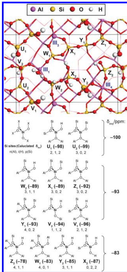
Figure 3. On the top, top view of the Si/ \text{Al}_2\text{O}_3 DFT model employed with \theta_{\text{OH}} = 5.4 \text{ nm}^{-2} , constructed from the silication of the (100) \gamma - \text{Al}_2\text{O}_3 surface. The terminology for Si and outermost surface Al atoms is given in black and blue, respectively. See Figure S2 and Table S4 (ESI) for more details on local environments and side views. On the bottom, schematic representation of each Si site with the DFT-computed ^{29}\text{Si} chemical shifts in parentheses and the number and the nature of second neighbors for each Si atom on the ASA model employed. The environment of Si is noted Si( n\text{Al} , i\text{H} , p\text{Si} ), by extension of the terminology from previous work; 89 n + i + p can be larger than four because of the significant ionicity of the framework (some oxygen are more than 2-fold coordinated). According to the decomposition, DFT calculated peaks were lumped into three subgroups centered around the experimental peaks: \delta < -96 \text{ ppm} ; -96 \text{ ppm} \leq \delta \leq -88 \text{ ppm} ; -88 \text{ ppm} < \delta .
