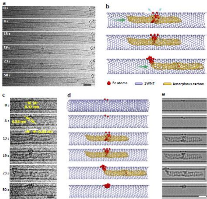
8 9 Figure 2 | Sequential AC-HRTEM images and corresponding simulations showing the first 10 and second stages of \gamma -Fe crystallite nucleation. a , AC-HRTEM raw images of the first stage 11 from 0 s to 13 s, ‘Diatomic Seed’ formation, and the second stage from 13 s to 50 s, the ‘Atom
