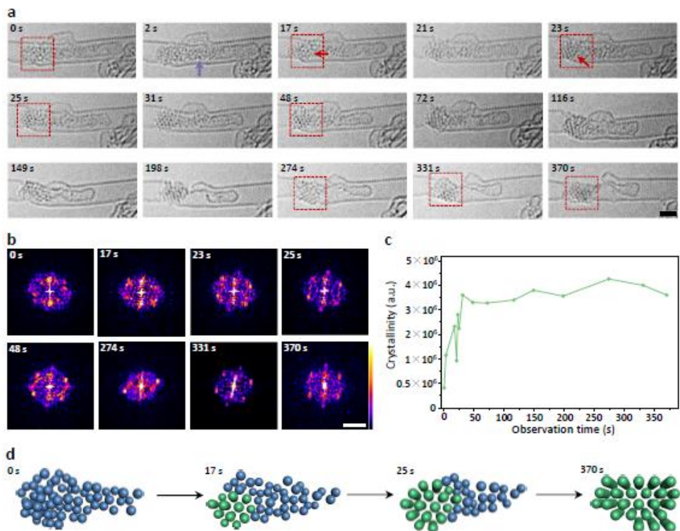
1 2 Figure 4 | E-beam stimulated nucleation of Au crystallite from the amorphous state. a, 3 Time-series AC-HRTEM images showing an amorphous Au cluster gradually transforming into 4 its crystalline structure under 80 keV e-beam irradiation. The formed crystallite is indicated by 5 red arrows; scale bar, 1 nm. b, FFT patterns of the corresponding areas framed by red dotted 6 boxes in a demonstrating the formation of the Au crystallite. Some Au atoms in this Au cluster 7 diffuse into the neighboring carbon nanostructure as indicated by the violet arrow; scale bar, 8 1/5 nm. c, Quantified crystallinity of the Au cluster during the nucleation in a and b. d, 9 Schematics of the gradual nucleation of the Au crystallite (the amorphous parts are shown in 10 blue, the crystalline parts in green).
