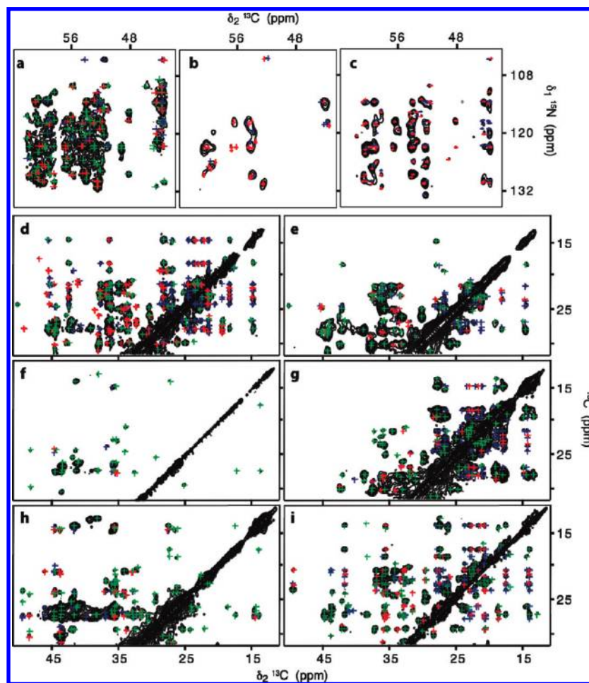
Figure 3. Extracts from spectra recorded on the different samples. (a) NHC, recorded on a uniformly ^{13}\text{C} – ^{15}\text{N} labeled sample; (b) NHC and (c) PAIN spectra recorded on ^{13}\text{C}/^{15}\text{N} mixed samples; (d) CHHC, recorded on a uniformly ^{13}\text{C} – ^{15}\text{N} labeled sample; (e) CHHC, recorded on a diluted, uniformly ^{13}\text{C} – ^{15}\text{N} labeled sample; (f) PDS, recorded on a diluted 2\text{-}^{13}\text{C} -glycerol-grown checkerboard sample; (g) PDS, recorded on a diluted 1,3\text{-}^{13}\text{C} -glycerol-grown checkerboard sample; (h) PDS, recorded on a 2\text{-}^{13}\text{C} -glycerol-grown checkerboard sample; and (i) PAR, recorded on a uniformly ^{13}\text{C} – ^{15}\text{N} labeled sample. Green, red, and blue crosses represent short-range (between residue i and j , |i - j| < 2 ), register ( |i - j| = 35, 36, \text{ or } 37 ), and other medium- or long-range restraints, respectively. Full views with assignments are shown in Supporting Information Figures S3–S12.
