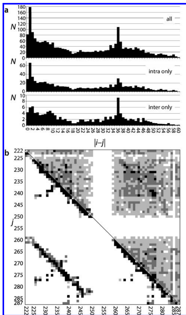
Figure 5. (a) Distance histogram of all ambiguous distance restraints used for the first run of structure calculation. The number N of restraints between residues i and j is counted for each possible distance |i - j| , where each ambiguity contributes the inverse of the number of possible assignments for the given restraint (i.e., the contribution of each peak is equal to 1). The sharp peak around |i - j| = 36 evidences the existence of the parallel \beta -sheets in both the intra- and intermolecular stacking. Note that intraresidual heavy-atom correlations were not used in the calculations. (b) Residue-residue plot with black, dark gray, and light gray squares indicating pairs of residues connected at least by 3, 1, and >0.1 “equivalent distance restraints”, respectively, where an “equivalent distance restraint” is the sum of distance restraints involving both residues weighted by the inverse of the number of assignment possibilities of the underlying peaks. In the upper right half, all distance restraint ambiguities used for the first run of structure calculation are shown, whereas the lower left part shows all assignment possibilities which were left for the final structure calculation.
