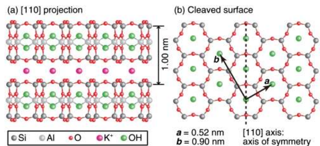
FIG. 1 (color online). Crystal structure of muscovite mica [KAl_2(Si_3Al)O_{10}(OH)_2] (Ref. [28]). (a) [110] projection. (b) Cleaved surface.
