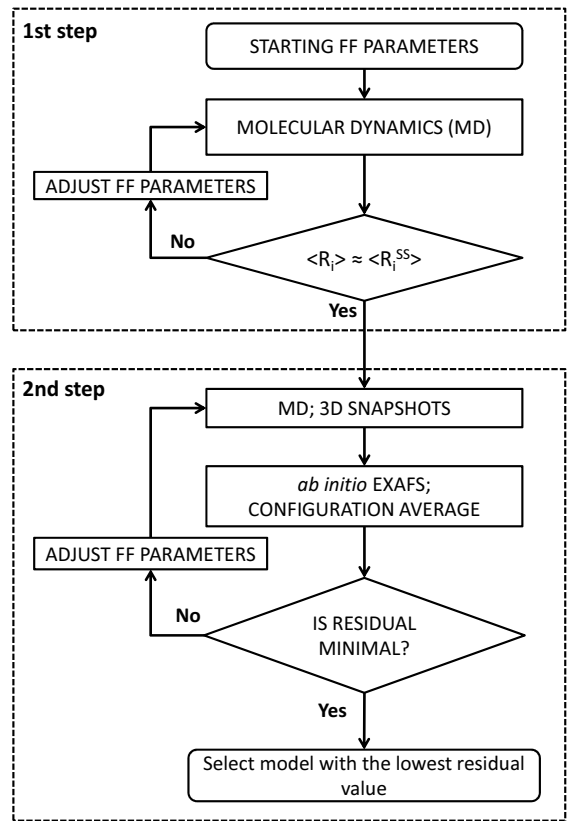
FIG. 6. A scheme of the MD-EXAFS calculation.
