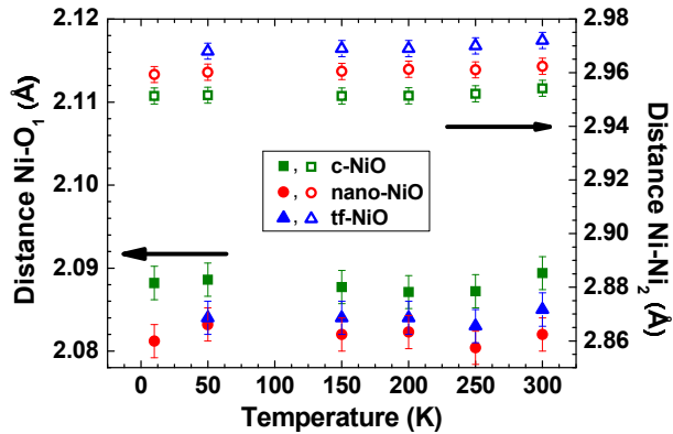
FIG. 4. (Color online) Temperature dependence of the average interatomic distances in the first ( \text{Ni-O}_1 ) and second ( \text{Ni-Ni}_2 ) coordination shells of nickel in c-NiO, nano-NiO and tf-NiO.
