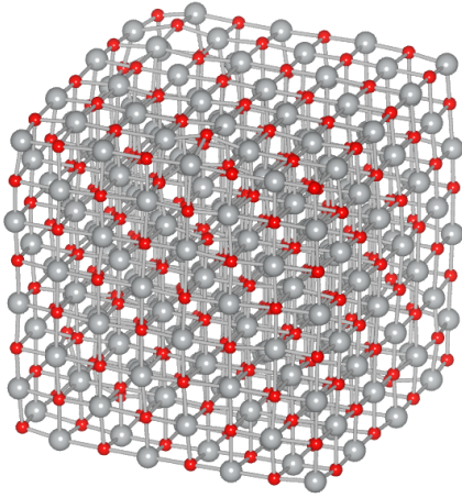
FIG. 7. (Color online) Example of the single MD snapshot of NiO nanoparticle with the size L = 9 and four nickel vacancies. Small red balls indicate oxygen atoms; large gray balls correspond to nickel atoms.
