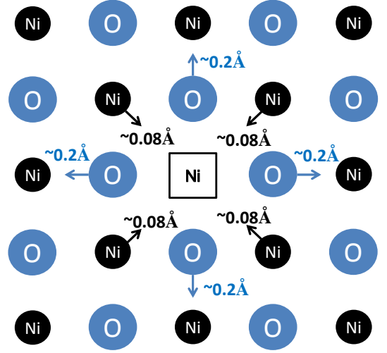
FIG. 8. (Color online) Schematic view of the nearest neighbor relaxation around a nickel vacancy in the bulk of nickel oxide according to our molecular dynamics simulations. Note that oxygen atoms move outwards, but nickel atoms move inwards to the nickel vacancy.
