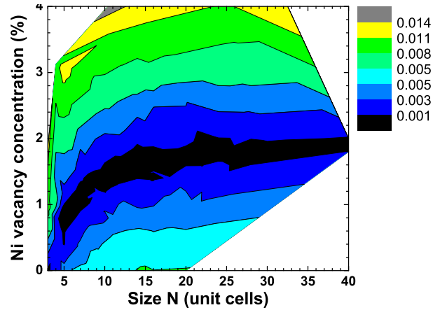
FIG. 9. (Color online) The dependence of the residual modulus value |\Delta R(\text{Ni-O}_1)| between the first shell interatomic distances, obtained for cubic NiO nanoparticles by conventional analysis method (See Fig. 4) and from the MD simulation, on the nickel vacancy concentration C_{\text{vac}} and the nanoparticle size L = Na_0 under imposed requirement that the second shell interatomic distance R(\text{Ni-Ni}_2) should coincide with the value, obtained by the conventional modeling procedure (See Fig. 4), within \pm 0.001 Å.
