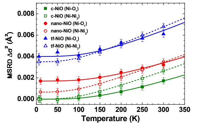
FIG. 3. (Color online) Temperature dependence of the mean-square relative displacements (MSRD) \sigma^2 for the first (Ni-O 1 ) and second (Ni-Ni 2 ) coordination shells in c-NiO, nano-NiO and tf-NiO relative to the MSRD value in c-NiO at T = 6 K. The Debye models are shown by lines. See text for the values of the characteristic Debye temperatures.
