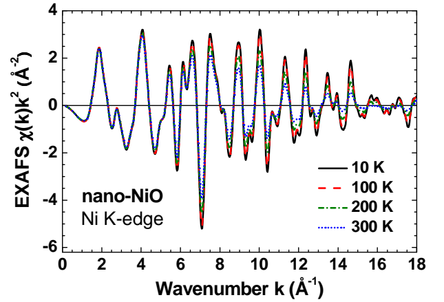
FIG. 2. (Color online) The Ni K -edge EXAFS spectra \chi(k)k^2 for nano-NiO at selected temperatures. Thermal disorder leads to the oscillations damping at high- k values.
