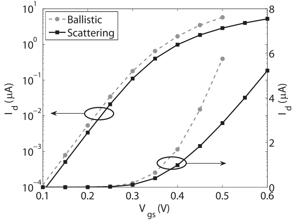
FIG. 4: Same as Fig. 3, but for a Si nanowire with a diameter d=2.5 nm.
