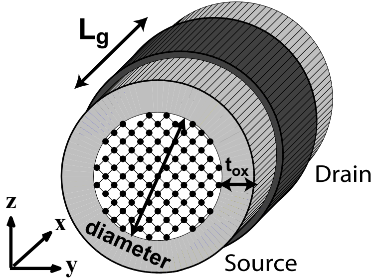
FIG. 1: Schematic view of a gate-all-around (GAA) circular Si nanowire field-effect transistor (NW FET) with a diameter d=2, 2.5, and 3 nm. The transport direction x is aligned with the \langle 100 \rangle crystal axis. The \text{SiO}_2 dielectric layer has a thickness t_{ox}=1 nm. The gate length L_g measures 15 nm while the source and drain contacts have a length of 12.5 nm and a donor doping concentration N_D=1e20 \text{ cm}^{-3} .
