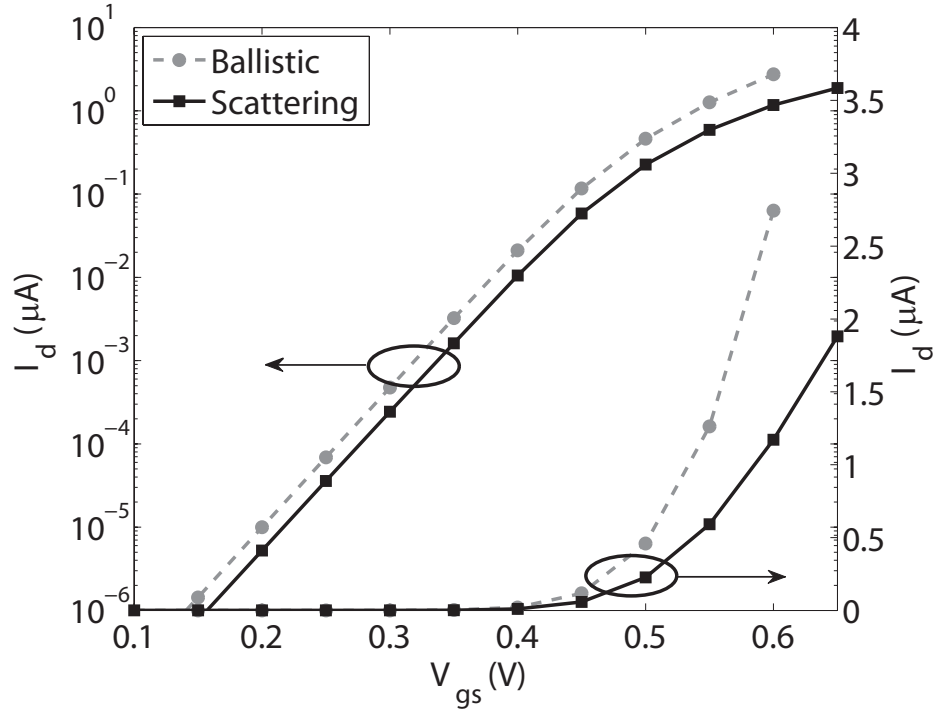
FIG. 3: Transfer characteristics I_d - V_{gs} at V_{ds}=0.6 V of a Si GAA NW FET with a diameter d=2 nm. The gray lines with circles refer to the ballistic current, the black lines with squares to the current with electron-phonon scattering.
