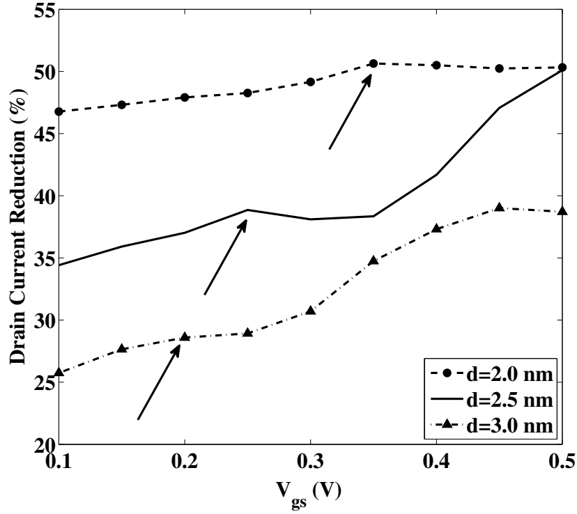
FIG. 6: Drain current reduction due to electron-phonon scattering at V_{ds}=0.6 V as function of V_{gs} in Si nanowires with a diameter d=2.0 nm (dashed line with circles), d=2.5 nm (solid line), and d=3.0 nm (dashed-dotted line with triangles). The ballistic I_{ball} and dissipative I_{scatt} currents of Fig. 3 to 5 are used to calculate (I_{ball}-I_{scatt})/I_{ball}*100 . The arrows indicate the threshold voltage in the ballistic simulations.
