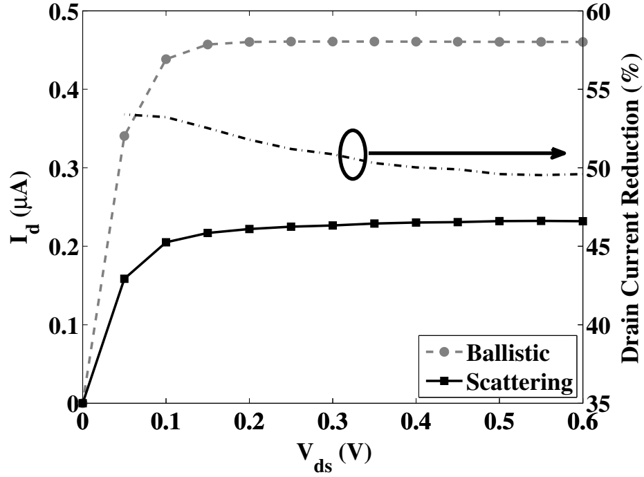
FIG. 7: Output characteristics I_d - V_{ds} at V_{gs}=0.5 V (left y-axis) of the Si GAA NW FET with a diameter d=2 nm. The gray lines with circles refer to the ballistic current, the black lines with squares to the current with electron-phonon scattering. The drain current reduction due to scattering is plotted on the right y-axis. It is defined as in Fig. 6.
