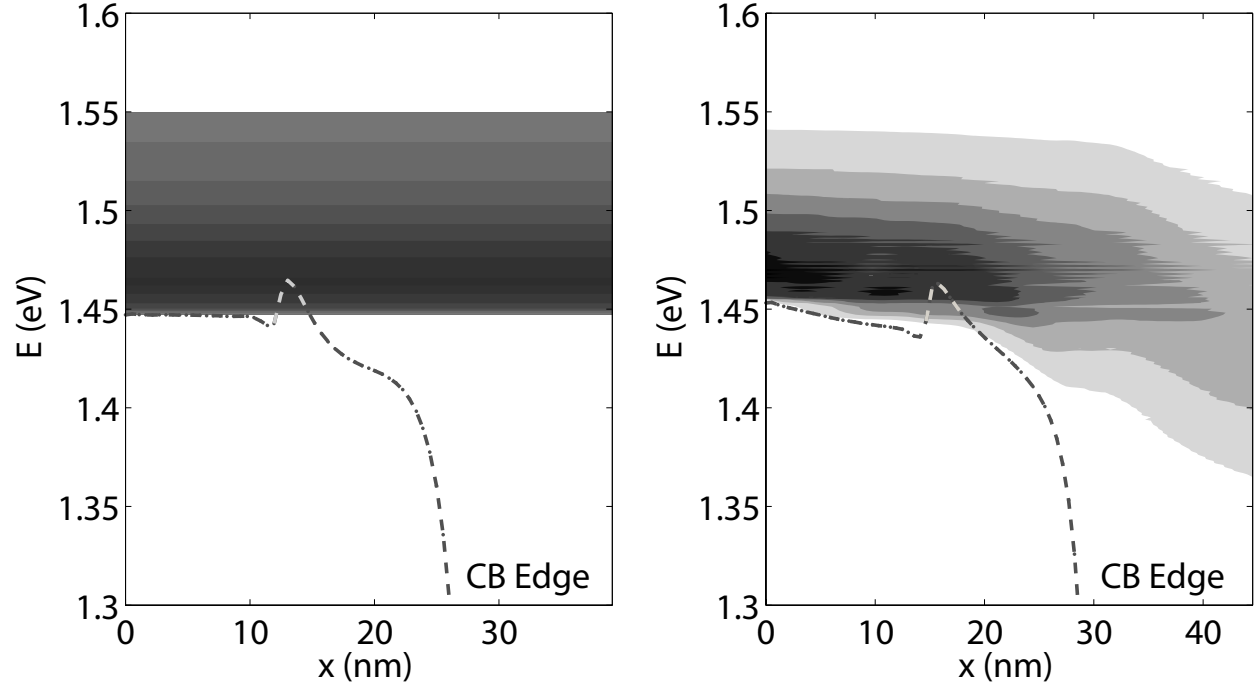
FIG. 10: Spectral current of the Si GAA NW FET with a diameter d=2.5 nm from Fig. 4 at V_{gs}=0.5 V and V_{ds}=0.6 V. The left subplot represents the ballistic current (homogeneous), the right subplot the current with electron-phonon scattering. The dashed lines indicate the position of the conduction band (CB) edge.
