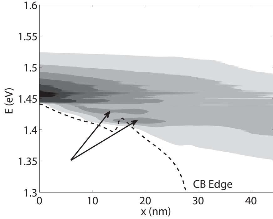
FIG. 12: Spectral current of the Si GAA NW FET with a diameter d=2.5 and electron-phonon scattering at V_{gs}=V_{ds}=0.6 V. The arrows indicate two regions with high current densities, separated by an energy difference of 15-16 meV.
