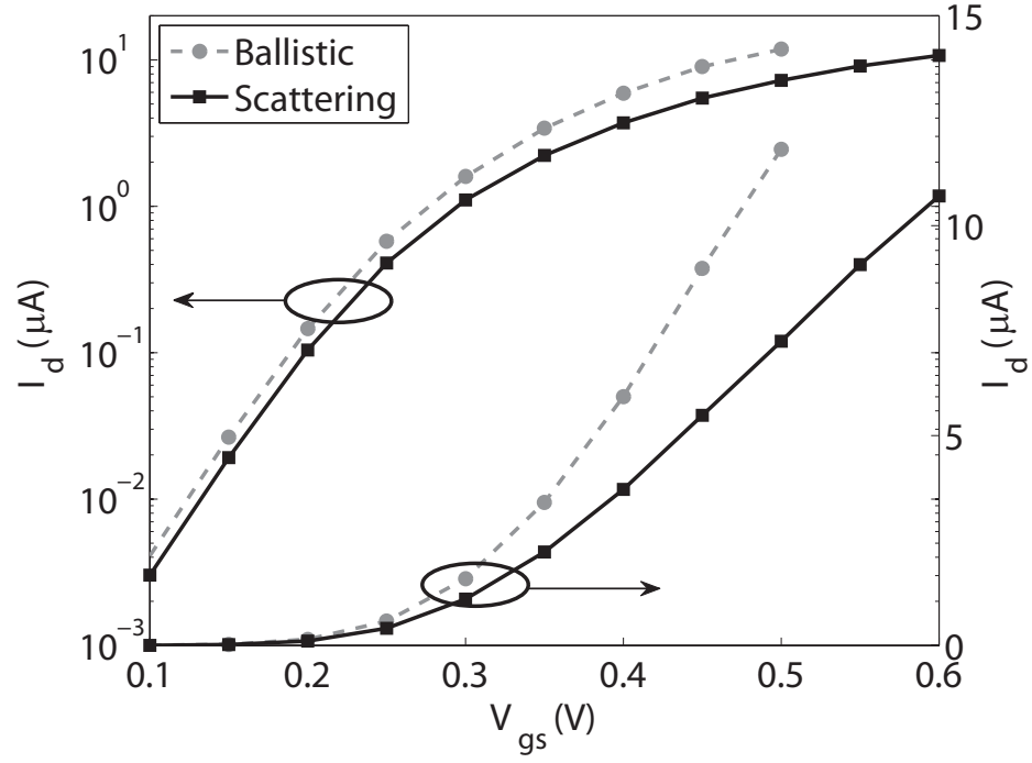
FIG. 5: Same as Fig. 3 and 4, but for a Si nanowire with a diameter d=3 nm.
