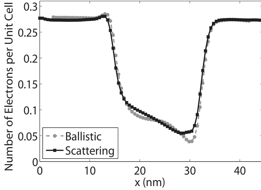
FIG. 9: Number of electrons per unit cell (ensemble of 4 atomic layers in the transport direction x ) for the Si GAA NW FET with a diameter d=2.5 nm at V_{ds}=0.6 V and V_{gs}=0.5 V. The gray line with circles depicts the ballistic electron density, the black line with squares the carrier density in presence of electron-phonon scattering. The number of doping atoms per unit cell in the source and drain contacts is 0.274.
