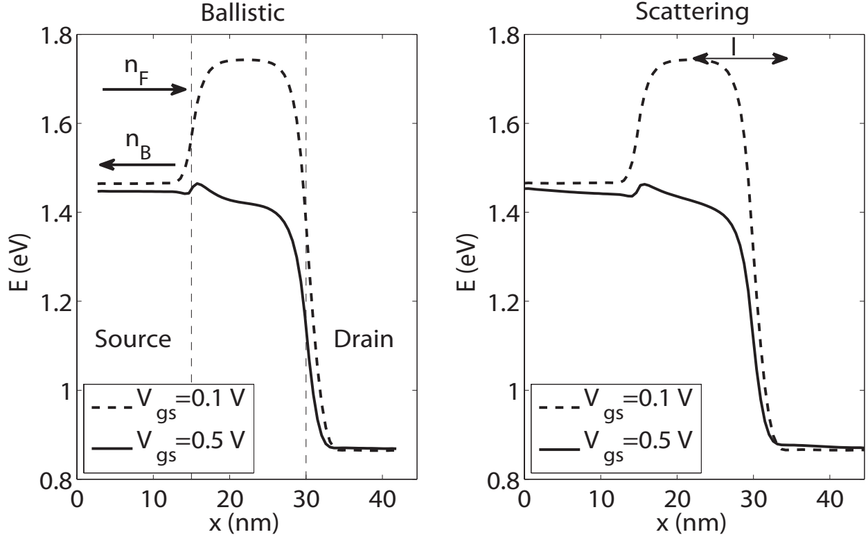
FIG. 8: Conduction band edges at V_{ds}=0.6 V, V_{gs}=0.1 V (dashed lines) and V_{gs}=0.5 V (solid lines) in the nanowire with d=2.5 nm. The band edges in case of ballistic transport are shown in the left subplot, those with electron-phonon scattering in the right subplot. The variable n_F ( n_B ) describes the electrons moving forwards (backwards) to (from) the gate, l is the critical length for backscattering 65 .
