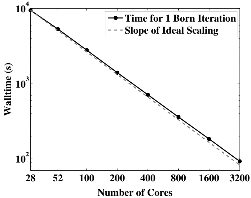
FIG. 13: Parallel execution time on a CRAY XT4 for the calculation of one Born iteration, i. e. for the solution of Eq. 1 to 4 and Eq. 14 for all the energies E on 28 to 3,200 cores. The test structure is a nanowire with n=2 nm and N_E=1,571 energy points. Each energy point is treated by four CPUs. Typically, 20 to 50 Born iterations are required to obtain the device current.
