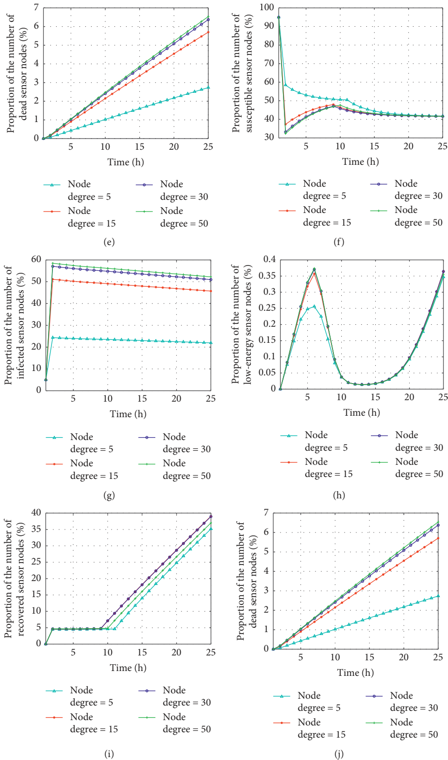
FIGURE 8: Evolution of sensor nodes with Logistic Growth in susceptible sensor nodes. (a) The quantity of susceptible sensor nodes with controllable input; (b) the quantity of infected sensor nodes with controllable input; (c) the quantity of low-energy sensor nodes with controllable input; (d) the quantity of recovered sensor nodes with controllable input; (e) the quantity of dead sensor nodes with controllable input; (f) the quantity of susceptible sensor nodes with uncontrolled input; (g) the quantity of infected sensor nodes with uncontrolled input; (h) the quantity of low-energy sensor nodes with uncontrolled input; (i) the quantity of recovered sensor nodes with uncontrolled input; (j) the quantity of dead sensor nodes with uncontrolled input.
