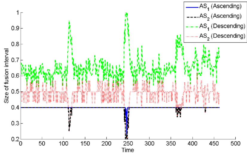
Fig. 9: Comparison of the sizes of the fusion intervals as obtained with the two attack strategies, optimization ( AS_1 ) and offset ( AS_2 ), and two schedules.
