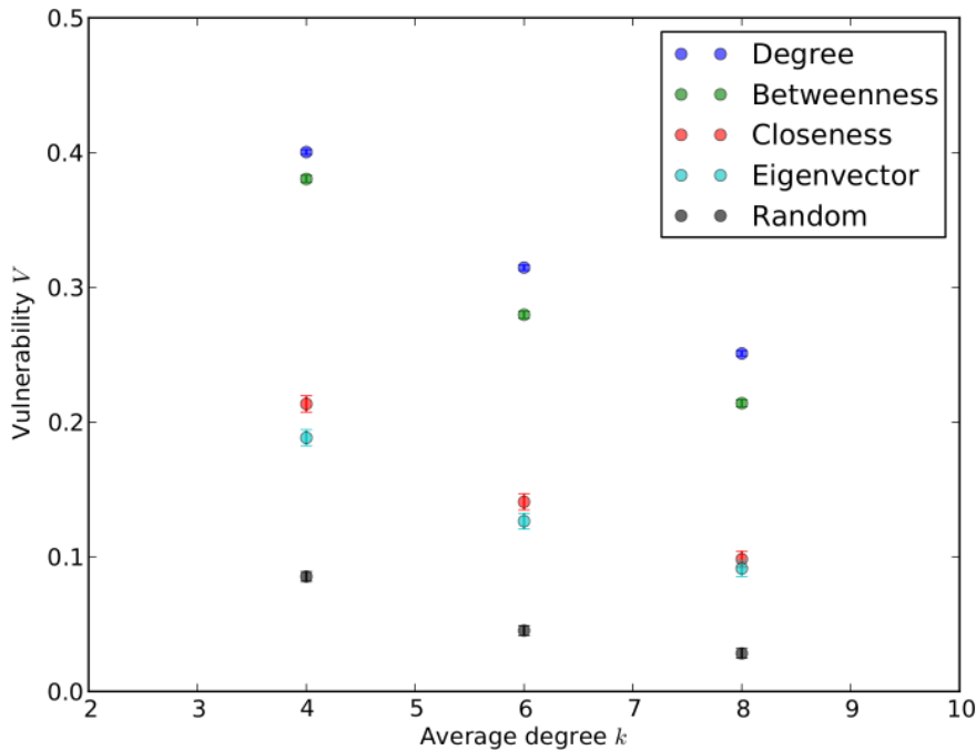
Figure 2. Variance in V-index for scale-free networks with N=10000 and different average degree k . The variance is based on ten different realizations of the network for each value of k , and the error bars represent the standard error. doi:10.1371/journal.pone.0059613.g002
