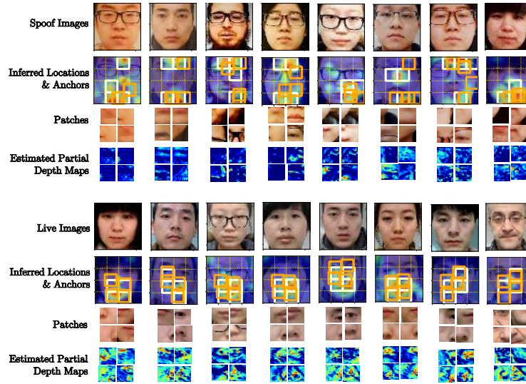
Fig. 5. Illustration of the model’s perception of live and spoof cases in OULU-NPU Protocol 1. The first four columns in the first row are print attack cases, followed by four replay attack cases.
