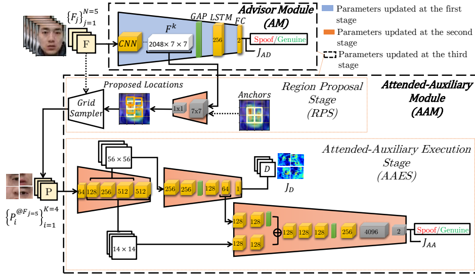
Fig. 2. Proposed framework constituted by interdependent attending modules. The AM plays a main role in providing the AAM with its experience in discerning spoof from genuine images. The AAM, in turn, draws attention to the received advice and sequentially processes images with reciprocal stages. For the architecture interpretation, the white, yellow, and green blocks represent feature blocks, sequential filters followed by a BatchNorm, and a rectified linear unit (RELU) activation function, respectively, each with a given size of 3 \times 3 and pooling layers. Apart from that, the gray blocks are depth-wise convolutions with size 7 \times 7 and point-wise convolutions with size 1 \times 1 . At the AAES, the patches proposed by the RPS are used to extract and to synthesize coarse to fine features with the help of the patch-driven depth map supervision D for PA detection. The figured is best viewed online in color.
