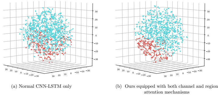
Fig. 4. 3D visualization of feature distribution extracted from the last layer next to the classification block of (a) a vanilla CNN-LSTM and (b) our model comprising the AM, intensified with SENets for channel interaction, and the AAM, enhanced with region attention. Red points represent genuine cases and blue points are spoof cases. The figure is best viewed online in color.
