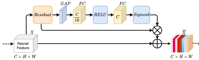
Fig. 3. Fundamental structure of a squeeze-and-excitation block, attached to each of the 101 residual blocks as a channel-wise enhancement submodule.
