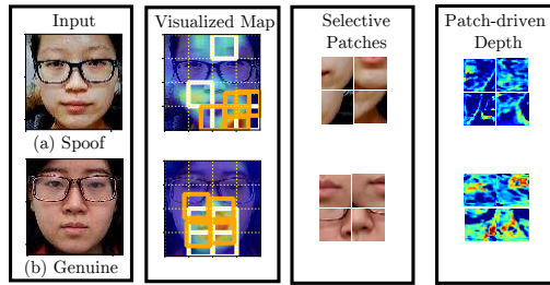
Fig. 1. Translation offsets of the orange regions, given the white initial locations of the AM, are thoroughly regularized based not only on binary supervision, but also on the attended auxiliary supervision in a multi-task learning manner.
