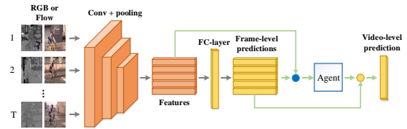
Figure 1: Flow-chart of our proposed method for action recognition. Each stream takes a sequence of frames or optical flow stacks as input. Then, an agent trained by deep reinforcement learning generates importance scores for all frames, which finds the attentions of the video for recognition.
