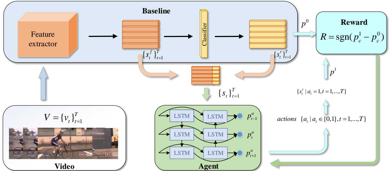
Figure 2: Process of training attention-aware sampling (AS) agent via deep reinforcement learning (spatial stream). The AS agent receives state \{s_t\}_{t=1}^T and takes action \{a_t\}_{t=1}^T to select part of the video. The feedback reward is computed based on the difference between the original video-level prediction p^0 and the new prediction p^1 .
