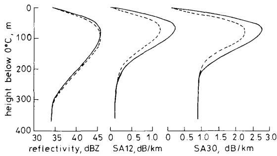
Fig. 3 Vertical profiles of reflection and specific attenuation in the melting layer
