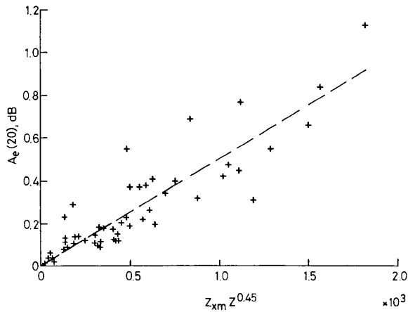
Fig. 6 Attenuation excess vs. radar reflection in, and below the bright band
