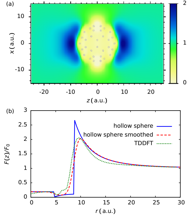
FIG. 21 (Color online) Field distribution of the streaking field near C_{60} (Wachter, 2014; Wais, 2014): (a) Local distribution in the x - z plane. The positions of the C atoms are indicated by the grey circles. (b) Normalized field distribution along the polar ( z ) axis, F(z)/F_0 , with F_0 the amplitude of the streaking field.
