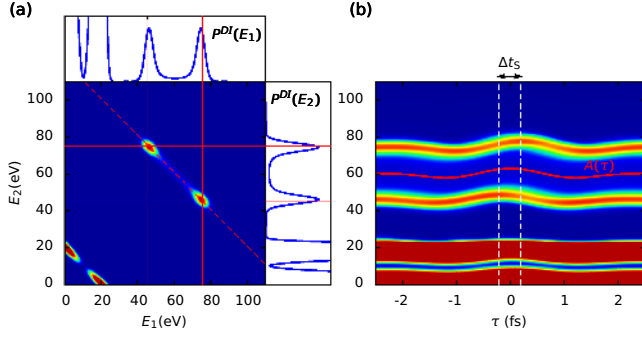
FIG. 27 (Color online) Simulation of two-photon double ionization of helium: (a) Joint two-electron energy distribution P^{\text{DI}}(E_1, E_2) for TPDI with \langle\omega_{\text{XUV}}\rangle = 100 eV and a pulse duration \tau_{\text{XUV}} of 500 as, emission back-to-back along the polarization direction ( \theta_1 = 0^\circ , \theta_2 = 180^\circ ). The panels above and on the right show the singly-differential energy distribution P^{\text{DI}}(\epsilon) after tracing out the energy of the second electron. (b) Streaking spectrogram from the integrated spectra P^{\text{DI}}(\epsilon_2) in (a) at different delay times \tau between the ionizing XUV pulse and the probing IR field ( \lambda_{\text{IR}} = 800 nm, I_{\text{IR}} = 4 \cdot 10^{11} W/cm ^2 , sine-squared envelope with a total duration of 6 fs).
