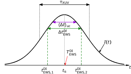
FIG. 28 (Color online) Illustration of time observables for two-electron emission in TPDI, schematically. The emission times of the first, t_{\text{EWS},1}^{\text{DI}} , and second electron, t_{\text{EWS},2}^{\text{DI}} , are measured relative to the arrival time (peak) t_a of the envelope of the attosecond XUV pulse ( t_a = 0 in the following) with temporal FWHM (in intensity) \tau_{\text{XUV}} . The relative emission delay between the two electrons is given by \Delta t_{\text{EWS}}^{\text{DI}} = t_{\text{EWS},1}^{\text{DI}} - t_{\text{EWS},2}^{\text{DI}} . Also shown is the estimate of the relative emission delay predicted for stochastic uncorrelated (uc) emission events \Delta t_{\text{uc}} and the joint emission time of the two-electron wavepacket T_{\text{EWS}}^{\text{DI}} .
