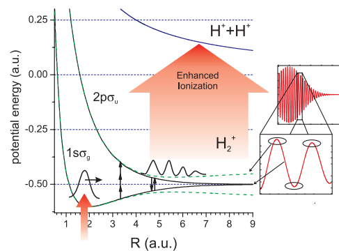
FIG. 1 (color online). Sketch of the time-dependent two-level system in H_2^+ . The two surfaces are shown for maximum (dashed line) and the zero crossing (solid line) of the laser field. Tunneling ionization of the neutral molecule creates a wave packet that rapidly moves towards the outer turning point. The two dissociation pathways, net-two-photon (absorption of 3 and reemission of 1 photon) and one-photon, interfere on the quasi-static upper state. Enhanced ionization samples the population on this surface at the field maximum of each half laser cycle.
