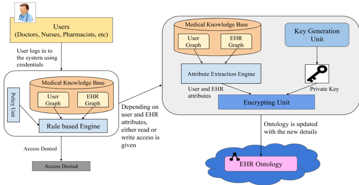
Fig. 1: System Architecture
