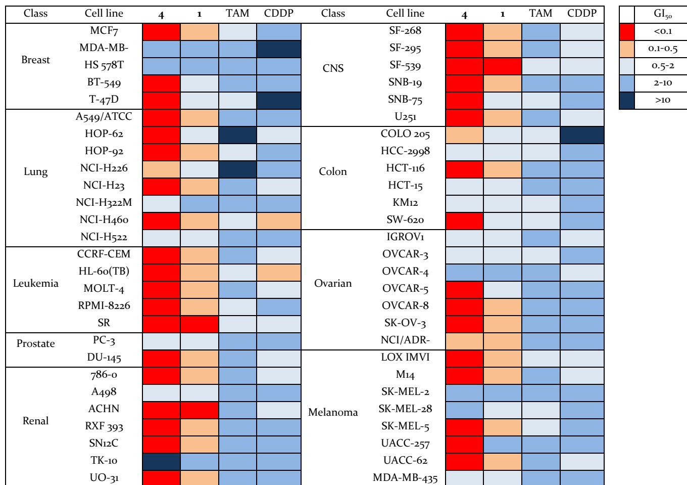
Fig. 4. Heat map for GI 50 values of 4, 1, TAM and CDDP. The cells were treated for 48 h at five concentrations ranging from 0.01 to 100 \mu M. GI 50 , 50% growth inhibition concentration. The deep red color indicates the highest activity, whereas the deep blue color represents the lowest activity.
