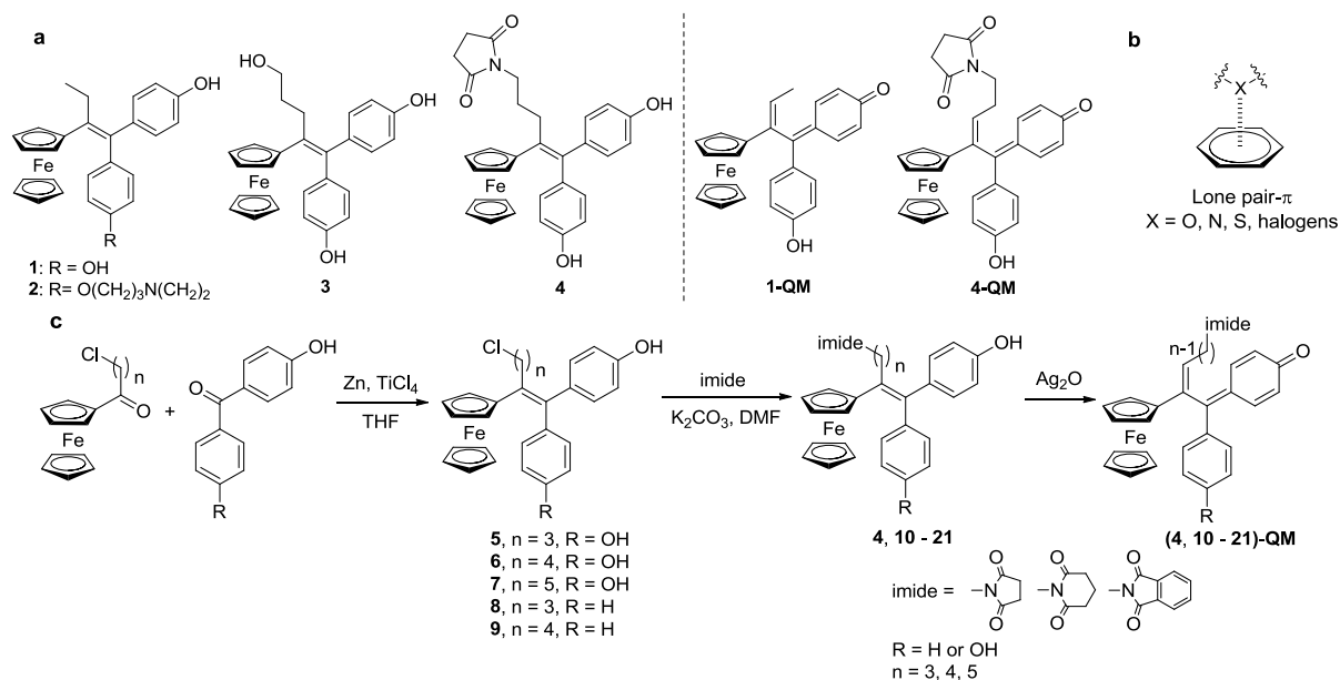
Fig. 1. (a) Ferrocifen derivatives and corresponding QMs. (b) The lone pair- \pi (lp- \pi ) interaction geometry. (c) Syntheses of imido-ferrocenols and their derived QMs.
