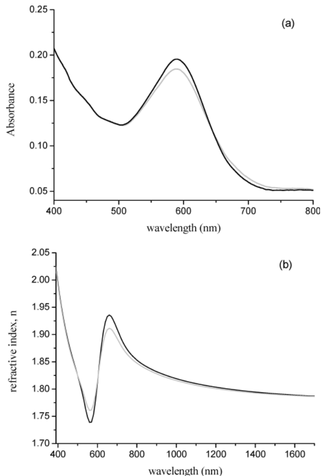
Figure 9. (a) Absorption spectra of a 50TiO 2 –50NiO film with Au NPs annealed at 500 °C measured in air (black line) and during exposure to 0.01% (v/v) H 2 S (light gray line) at an OT of 350 °C. The figure highlights the effect of gas exposure on the surface plasmon resonance frequencies of Au NPs (500–750 nm region). (b) Refractive index dispersion curves of a 70TiO 2 –30NiO film with Au NPs annealed at 500 °C before H 2 S exposure (black line) and after the “freezing” process (light gray line).
