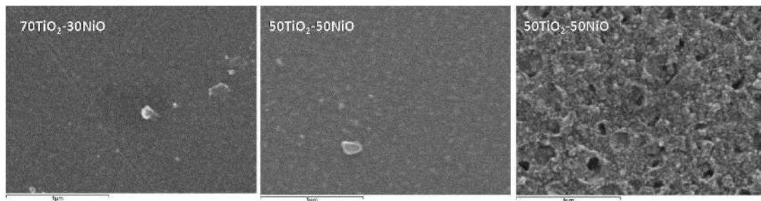
Figure 3. Bright field SEM images of the surface of different films containing Au NPs annealed at 500 °C. The scale bar is 1 \mu\text{m} .
