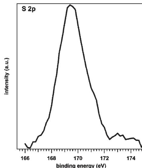
Figure 13. XPS S 2p region of the Au-doped 70\text{TiO}_2\text{--}30\text{NiO} film annealed at 500\text{ }^\circ\text{C} after the exposure to \text{H}_2\text{S} .
