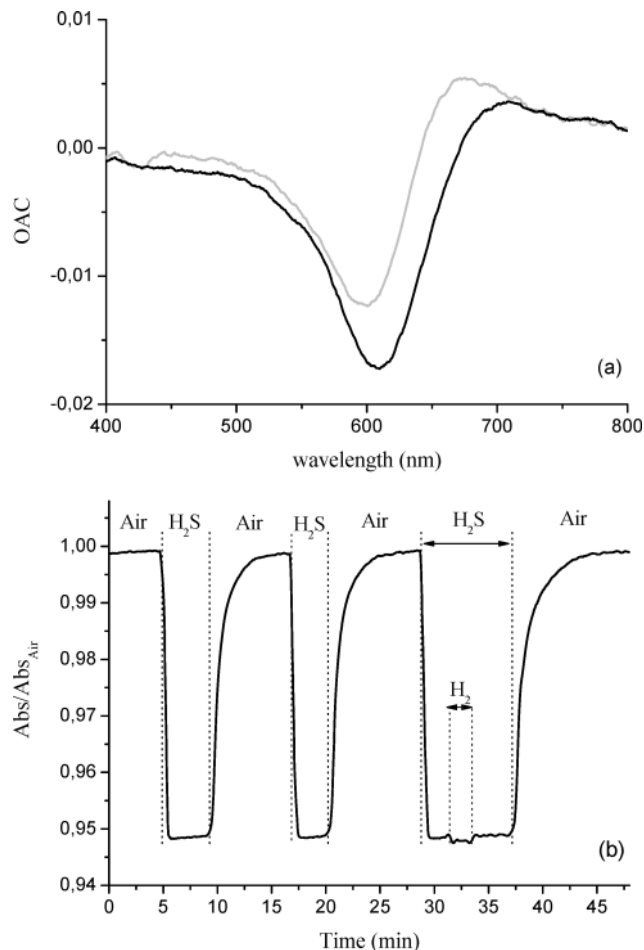
Figure 11. (a) Optical absorbance change ( OAC = A_{\text{gas}} - A_{\text{air}} ) of a Au-70TiO 2 -30NiO nanocomposite film annealed at 500 °C (gray line) and 600 °C (black line) after being exposed to 0.01% (v/v) H 2 S at an operative temperature (OT) of 350 °C. (b) Dynamic response at 605 nm of a Au-70TiO 2 -30NiO film annealed at 600 °C under exposure to an air-0.01% H 2 S-air-0.01% H 2 S-air-0.01% H 2 S/1% H 2 -air cycle at an OT of 350 °C.
