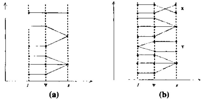
Figure 1: Illustrations of two measures l and g . A link between two points indicates that the function values are the same on domain \Psi . In (a), l is strictly consistent and more discriminating than g . In (b), l is not strictly consistent or more discriminating than g . Counter examples on consistency (denoted by X in the figure) and discriminaneity (denoted by Y) exist here
