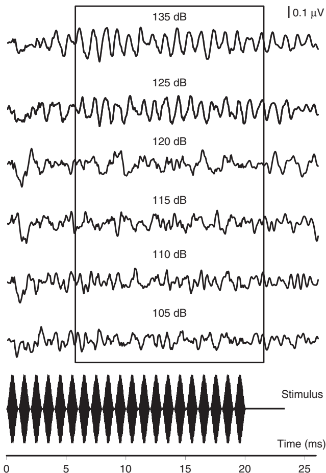
Fig. 4. Envelope following response (EFR) to a 150 kHz SAM stimulus from 105 to 135 dB re. 1 \mu Pa. The box indicates the 16 ms analysis window for the FFT.
