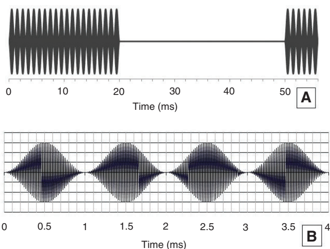
Fig. 2. (A) Sinusoidally amplitude modulated (SAM) tone stimulus used during the audiogram acquisition (150 kHz carrier frequency). (B) A 4 ms close-up of the same signal.
