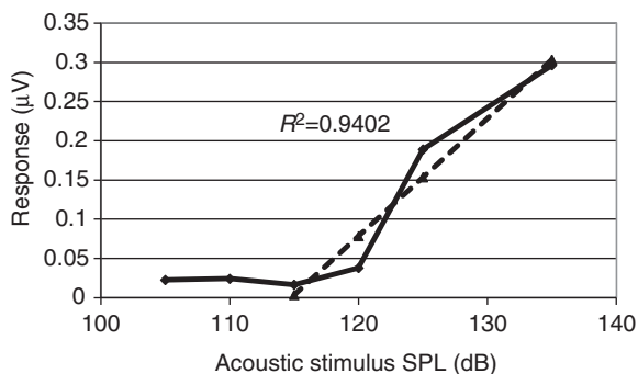
Fig. 6. Plot of the EFR amplitude at 1 kHz versus the corresponding acoustic stimulus sound pressure level (SPL) for the 150 kHz tone (solid line) and the linear regression (dashed line) calculated from 115 to 135 dB. The threshold was estimated as the intersection of the regression line with the zero value.
