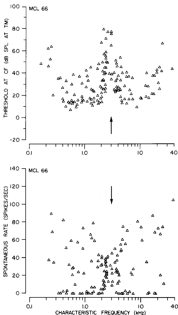
FIG. 5. Comparison of spontaneous rates and thresholds at CF in one acoustically traumatized animal. Threshold at CF was determined by the automated tuning-curve algorithm at a criterion of 1. This animal was exposed to narrow-band noise centered at 3 kHz (bandwidth of 50 Hz) for two hours at a sound pressure of 108 dB SPL (rms).
