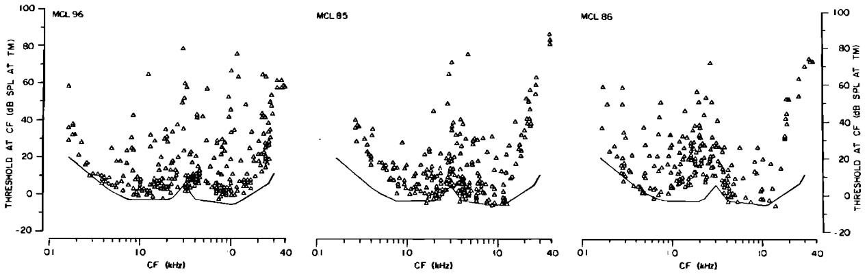
FIG. 2. Distribution of thresholds at CF obtained in three different cats. Each panel plots the threshold at the CF for each of the units encountered in one animal. For each unit, the "threshold" is that value obtained by the automated tuning-curve paradigm with a criterion of 1. The case in the left panel (MCL96) was one of the animals raised in the soundproofed room. The other two cases were cats from the population routinely available to us as experimental animals. Superimposed on the data from each animal is the "best-threshold curve," or BTC (see text). Since the BTC has been smoothed, some of the data points in MCL85 and 86 fall a few decibels below the curve. In this and all subsequent figures the sound pressure levels are expressed in decibels re 0.0002 \text{ dyn/cm}^2 , as measured near the tympanic membrane (TM).
