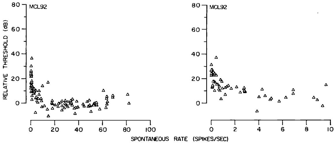
FIG. 12. Relation between spont and relative threshold in one of the routine-normal animals. All methods of data gathering and display are as described in the caption for Fig. 10.
