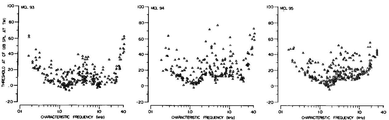
FIG. 3. Distribution of thresholds at CF seen in three of the chamber-raised cats. Since the thresholds in these three cases were determined by the automated tuning-curve paradigm at criterion 0, the BTC from Fig. 2 cannot be directly compared to these data.
