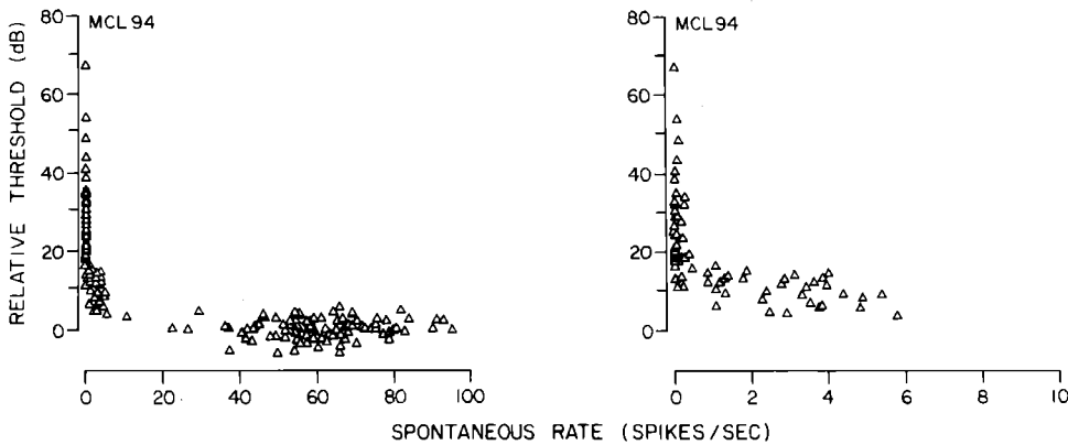
FIG. 10. Relation between spont and relative threshold in one of the chamber-raised animals. In the right panel the data from the low-rate units are displayed on an expanded horizontal scale. The relative threshold of each unit is the difference between its threshold at CF and the average threshold at CF of all the units from the same ear with similar CF and with rates of spontaneous discharge greater than 18 spikes/s. The normalization curve describing the average threshold as a function of CF was derived by dividing the CF continuum into 40 logarithmically spaced frequency bins, averaging the thresholds at CF for all the "high-spont" units within each CF bin and interpolating between the 40 mean-threshold values thus derived. Excluded from these scatter plots are those units with CF below 0.4 or above 15 kHz. Absolute threshold measurements were made with the automated tuning-curve program at criterion 0.
