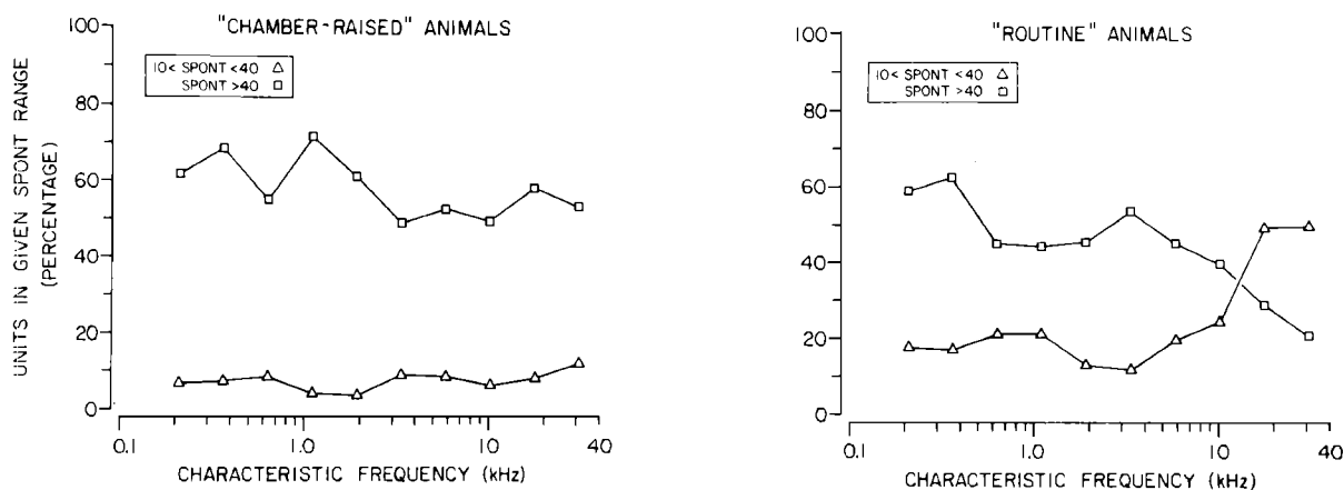
FIG. 7. Compression of the spont rate distribution at high CF in routine animals. The data in the left panel are from three chamber-raised cats (MCL93, MCL94, and MCL96). The data on the right are from 14 animals among those routinely available from local suppliers (MCL14, 47, 49, 75, 79-86, 89, and 90). To make each curve, the units in the sample were divided according to CF into ten logarithmically spaced frequency bins. Each box represents the percentage of units in that CF bin which had spont greater than 40 spikes/s; each triangle represents the percentage of units with spont between 10 and 40 spikes/s. Each symbol is placed in the center of the appropriate CF bin.
