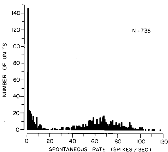
FIG. 9. Histogram of spontaneous rates sampled from the three most sensitive chamber-raised cats (MCL93, 94, 96). The bin width for the histogram is 1 spike/s. The "N" refers to the number of units in the sample.
