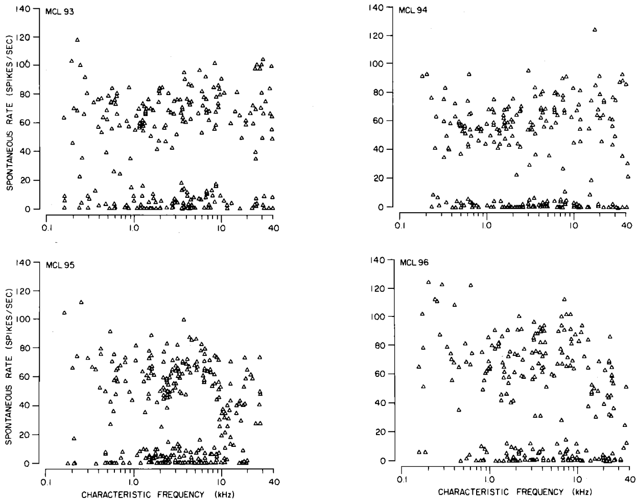
FIG. 6. Distribution of spontaneous rates as a function of CF as seen in each of the four chamber-raised cats. Each panel contains the data from all the units in that particular animal for which electrode contact was maintained long enough to procure both a tuning curve and a 30-s sample of spontaneous activity.
