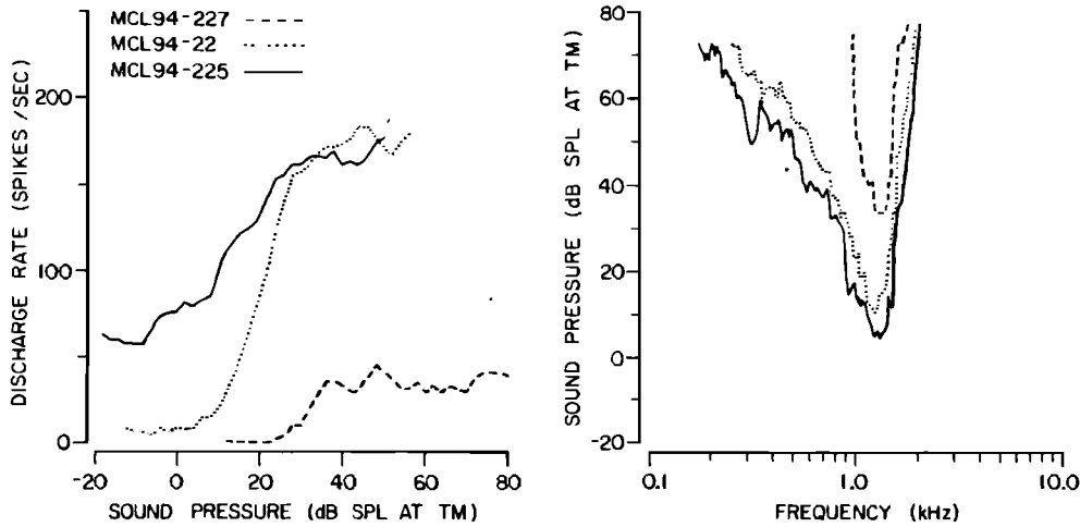
FIG. 16. Typical rate-level functions at the CF for units from the three spont classes in one of the chamber-raised animals. The tuning curves for the three units (criterion 0) are shown in the right-hand panel. The rate-level functions (left) have undergone three-point smoothing. The spont rate for units 227, 22, and 225 were 0.03, 3.83, and 56.3 spikes/s, respectively.
