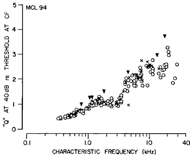
FIG. 14. Tuning curve "Q" as a function of CF with coding for spont rate. "Q" is measured at 40 dB re threshold at CF and is defined as the ratio of the characteristic frequency to the bandwidth of the tuning curve. Solid triangles represent low-spont units, crosses represent medium-spont units, and open circles represent high-spont units. The data are taken from one of the chamber-raised animals.
