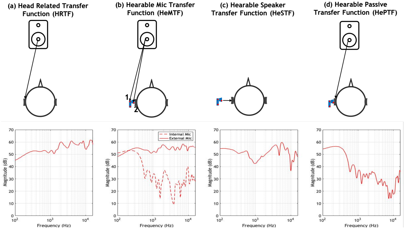
Fig. 5. Transfer functions for AR/MR audio. Example of magnitude response measured: (a) HRTF at the eardrum of the dummy head with open ear; (b) HeMTF at the external and internal microphones of hearables; (c) HeSTF from hearables speaker to eardrum of the dummy head; (d) HePTF at the eardrum of the dummy head with hearables worn on the ear
