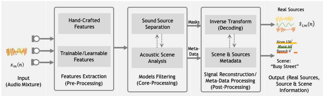
Fig. 6. An example overview architecture of acoustic scene analysis block, which takes audio mixture captured from hearables microphones as input, followed by feature-extraction, processes the extracted features to compute source masks or analyze the acoustic scene, and performs post-processing to reconstruct separated source signals and extract associated meta information like source type, spatial direction, and scene information as outputs.
