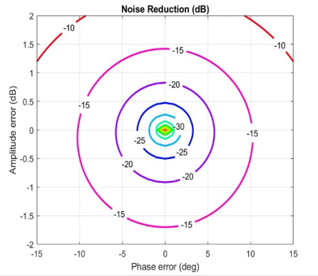
Fig. 11. ANC Performance as a function of amplitude error (in dB) and phase error (in deg)
