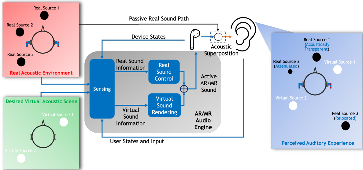
Fig. 3. Signal processing blocks for AR/MR audio. Three major blocks namely, sensing, real sound control and virtual sound rendering, along with their inputs and outputs are shown, along with an AR/MR audio use-case example.
