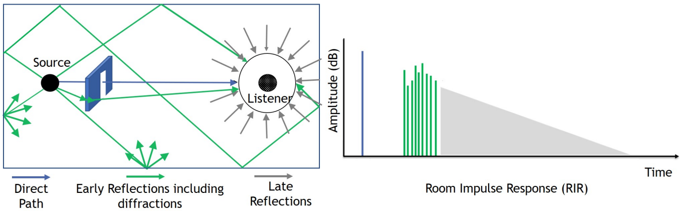
Fig. 7. Illustration of construction of typical room impulse response in an environment from source to listener via direct path (blue), early reflections (green), and late reflections (gray)
