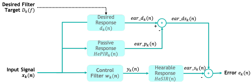
Fig. 10. Control filter calculation for a single source. The summation shown in figure is an acoustic summation.
