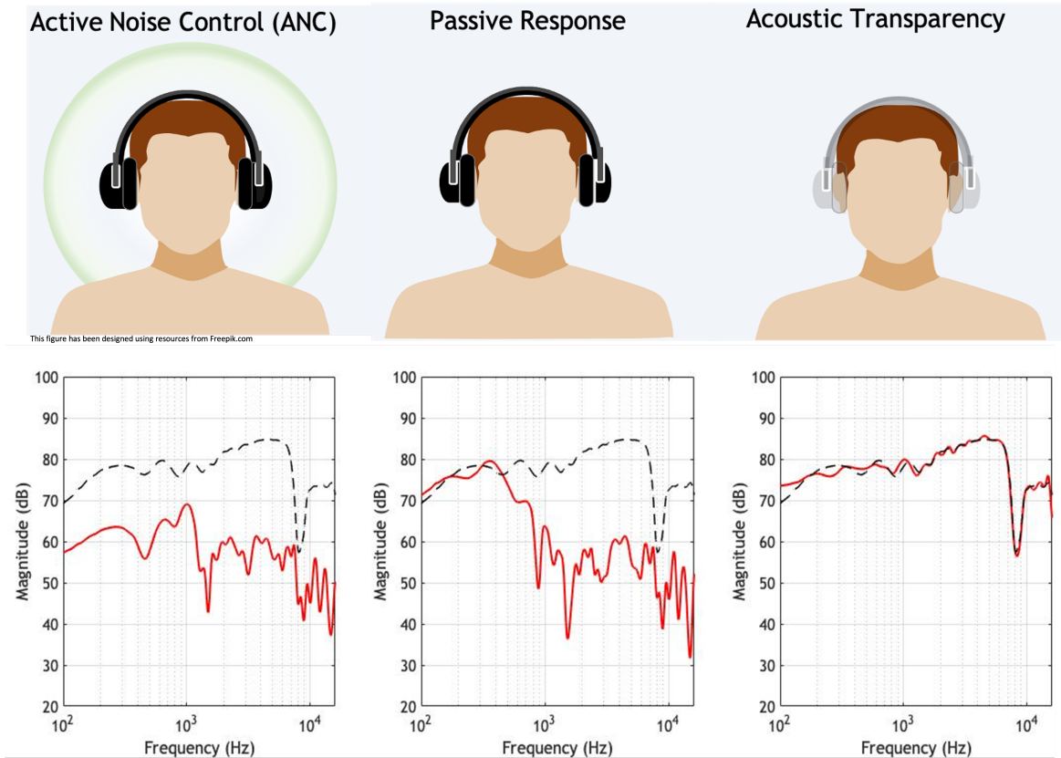
Fig. 9. Real sound control listening modes with examples of the responses at ear under these modes (solid red curve) in comparison to the open-ear response (dashed black curve).
