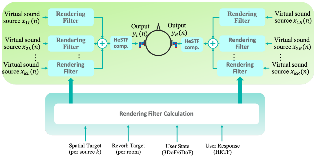
Fig. 12. Basic framework for virtual sound rendering in AR/MR audio. Rendering filter block performs room auralization using BRIR or delay networks, based on the inputs from Sensing.
