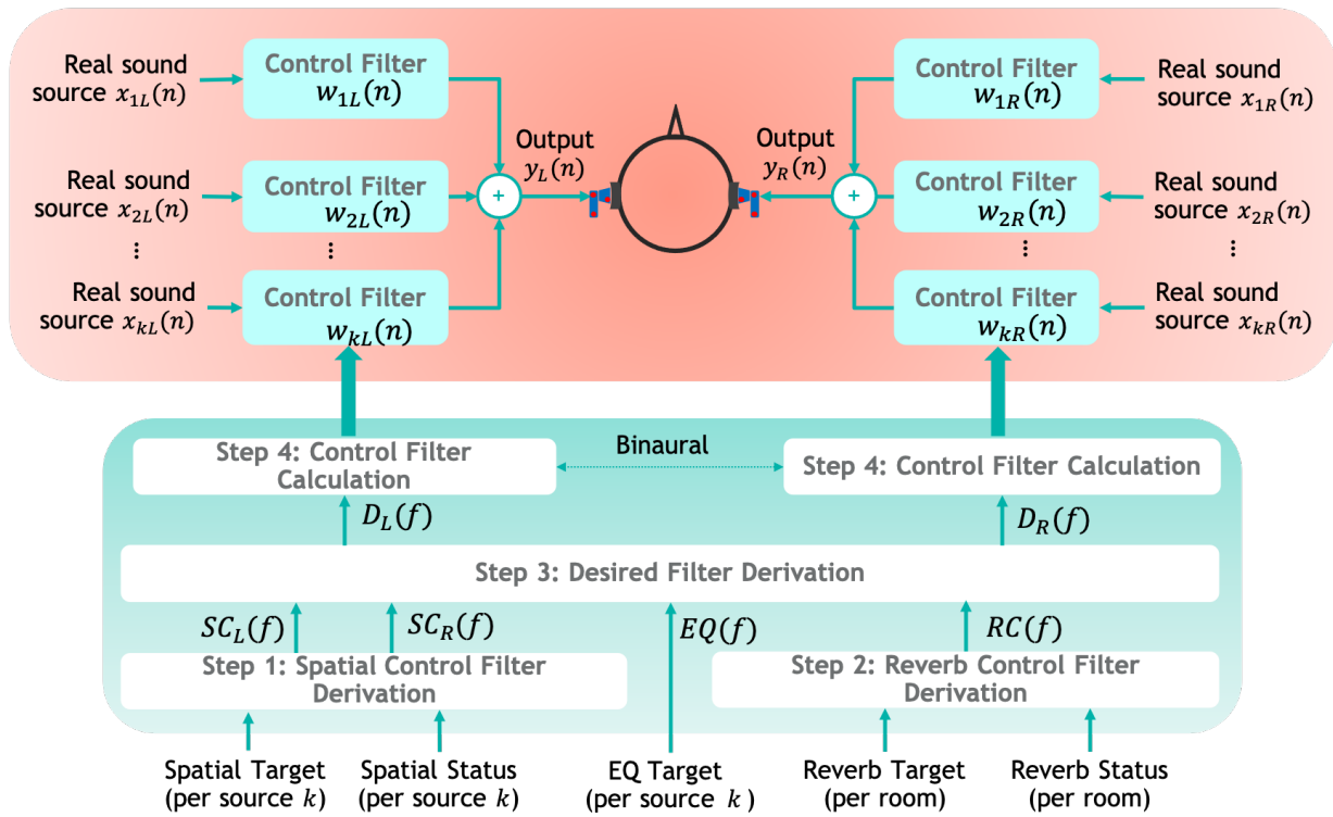
Fig. 8. Real sound control of multiple sources with derived control filters (shown inside orange box). A control filter is derived for each channel (left/right), and each real sound source. The four steps for computation of control filters are shown (inside green box).
