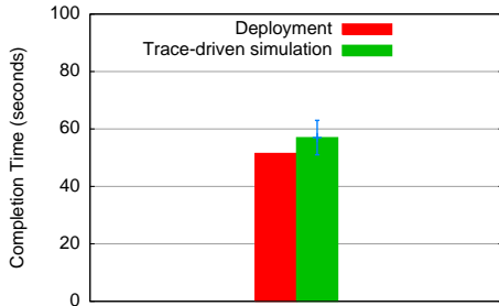
(a) Completion time
