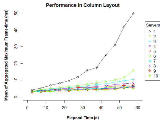
Fig. 5. Performance of increasing numbers of servers with an accumulating number of objects (in column layout)
