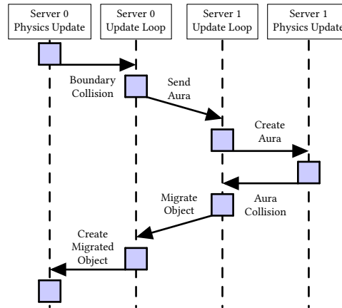
Fig. 2. Aura and migration sequence diagram
