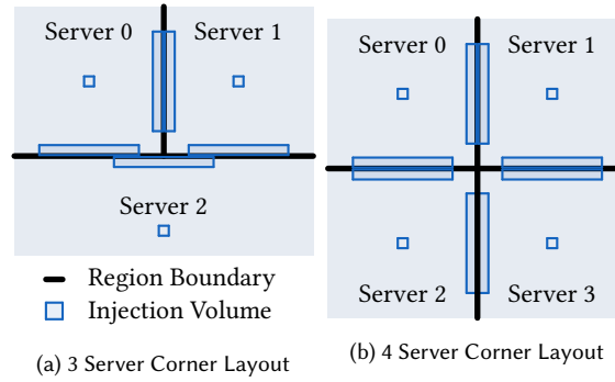
Fig. 6. Corner Layouts
