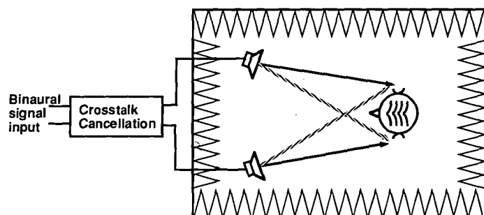
Fig. 5. Transaural playback of binaural recordings requires cancelation of interaural crosstalk by using a filter before the loudspeakers.
