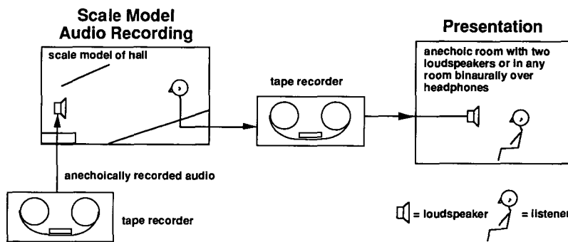
Fig. 8. Basic principles of a traditional system for direct acoustic scale model auralization.
