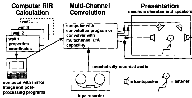
Fig. 6. Basic principles of a system for computed multispeaker auralization.
