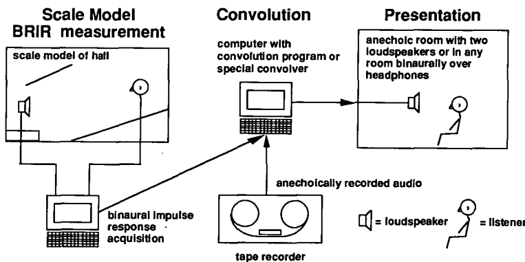
Fig. 9. Basic principles of a system for indirect acoustic scale model auralization.
