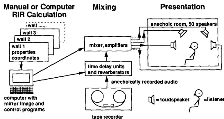
Fig. 7. Basic principles of a system for simplified computer multispeaker auralization using time delay units, reverberators, and mixer instead of detailed convolution of the audio signals.
