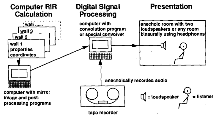
Fig. 1. Basic principles of a system for fully computed auralization.
