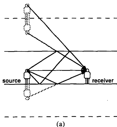
Fig. 2. Mirror-image model (a) requires generation of many image sources to adequately model the sound field. Equivalently ray tracing (b) requires many densely radiated rays to adequately model the sound field.
