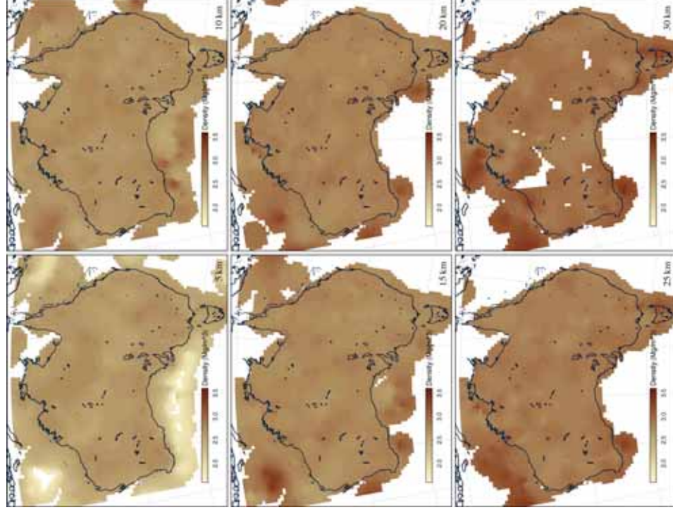
Figure A1. Distribution of density ( \rho ) for the AusREM crustal model at: (a) 5 km depth, (b) 10 km depth, (c) 15 km depth, (d) 20 km depth, (e) 25 km depth, (f) 30 km depth.
