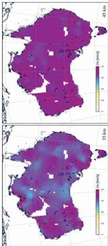
Figure 12. S wavespeed distribution for the AusSREM crustal model at: (a) 35 km depth, (b) 45 km depth. Receiver function constraints are shown by diamonds, plotted using the same colour scale as the background model.
