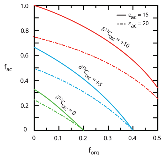
Fig. 2. Contours of \delta^{13}C of DIC as a function of f_{org} and f_{ac} for global average values of \epsilon_{ac} of 15 and 20‰, assuming that the carbon cycle is in steady state, and neglecting imbalances in other inputs, based on Eq. 2.
