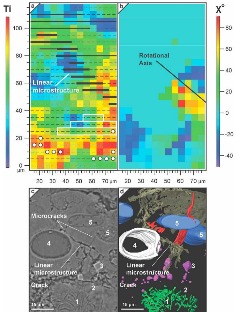
Figure 13. Highly altered basaltic glass of the fractured lapillus, 102.6-m depth (Figures 7b–7d and 10). (a) Grid of X-ray microfluorescence (Ti) analyses, at 5- \mu\text{m} step size, 60 \times 120\text{-}\mu\text{m}^2 area, showing sites of randomly oriented nanocrystalline clay mineral d spacing (dashed lines), a 50 \times 20\text{-}\mu\text{m} zone of nanocrystalline clay mineral exhibiting crystallographic preferred orientation (heavy black lines), coarse analcime (white outlines), and Al-tobermorite (white circles). (b) The crystallographic preferred orientation of the (001) 14.5- \text{\AA} peak of the nanocrystalline clay mineral (Figure 13a) rotates over an arch segment ( \chi ) of +50^\circ to -20^\circ along an axis that parallels the linear microstructure (see, also, Figures 7c and 7d). (c, d) Spatial relationships shown by micro-computed tomography analysis: olivine (1, green), Al-tobermorite (2), analcime (3, purple), nanocrystalline clay mineral (gray), empty vesicle (4, white), and vesicles filled with zeolite and Al-tobermorite (5, blue).
