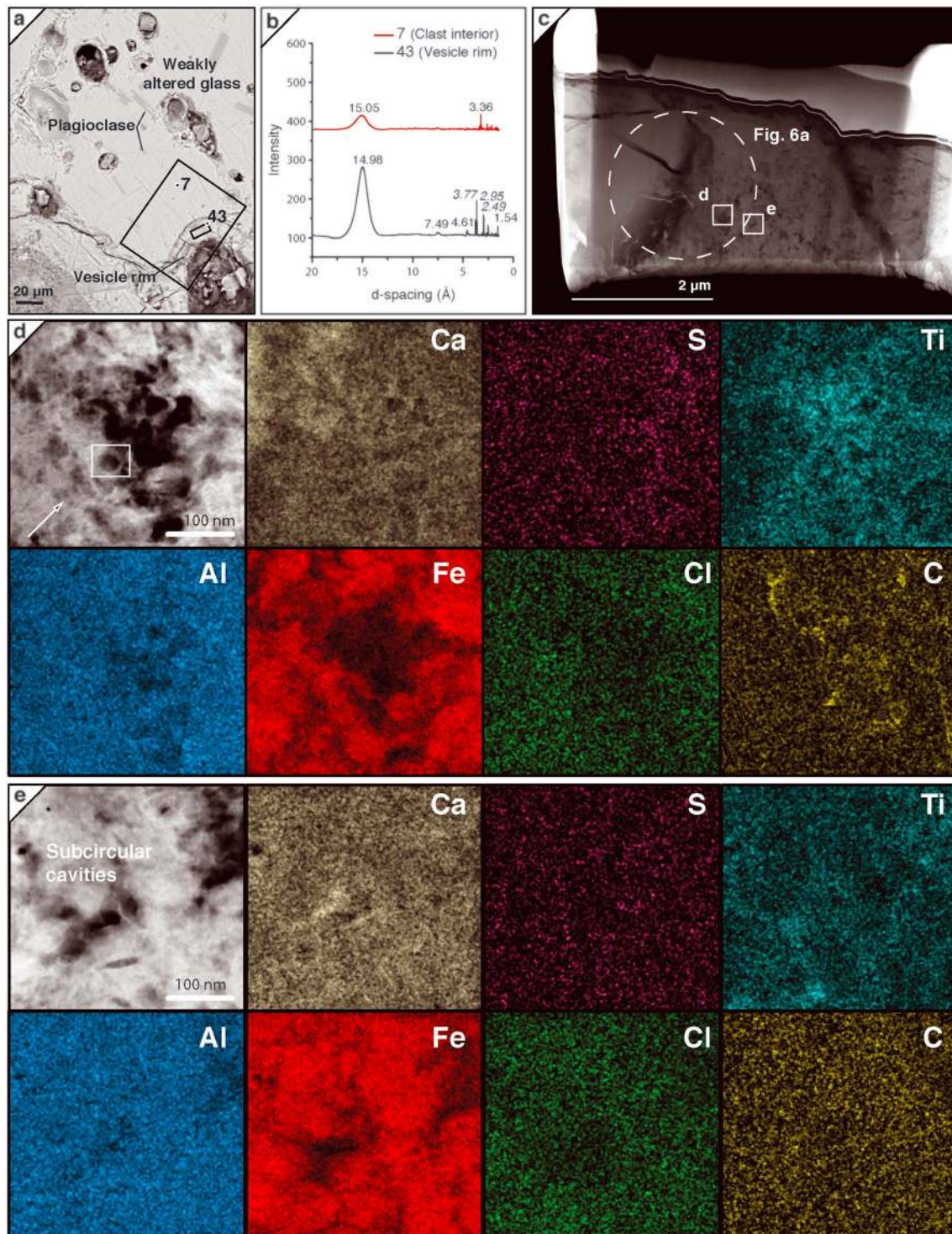
Figure 5. Basaltic lapillus, 137.9-m depth, showing investigations of altered glass. (a) Scanning electron microscopy-backscattered electron image, sites of X-ray microdiffraction ( \mu XRD) analyses and focused ion beam (FIB) lift out. (b) Intensity versus d spacing plot for \mu XRD analyses (#7 [red] and #43 [black]), including plagioclase [shown in italics ]. (c) FIB lift out, site of Raman spectra (Figure 7a). (d) Scanning transmission electron microscopy-energy dispersive X-ray spectrometer (S/TEM EDS) elemental maps, white rectangle indicates a subcircular cavity along the left edge of the vesicle and very fine nanoscale cavities nearby (arrow). (e) S/TEM EDS elemental maps, area of larger nanoscale subcircular cavities.
