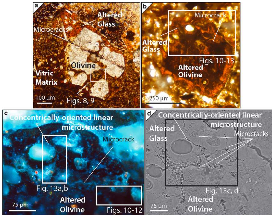
Figure 7. Fractured lapilli, with olivine crystals enrobbed in altered basaltic glass. (a) Mainly intact olivine, 137.9-m depth, and subcircular microstructures in altered glass, petrographic image (Figures 8 and 9). (b) Strongly altered olivine, 102.6-m depth, with a 75- to 100- \mu\text{m} altered glass rim, petrographic image (Figures 10–13). (c) Ultraviolet-excited native fluorescence image of a detail of (b). Note that larger fluorescent areas are superglue adhesive. (d) X-ray tomograph of (c), showing the area of micro-computed tomography analysis (Figure 13).
