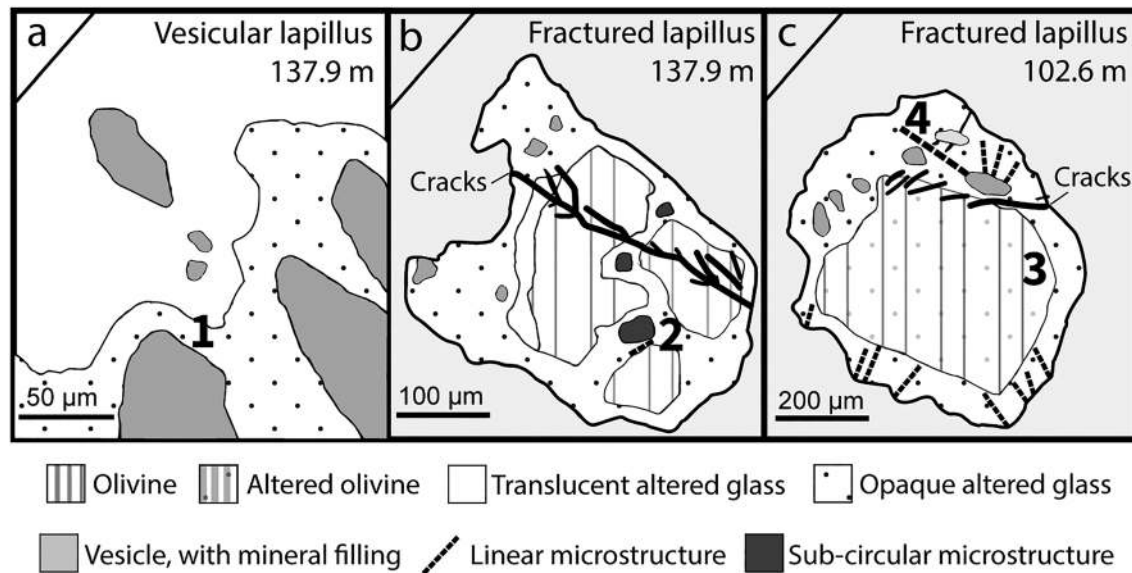
Figure 2. Examples of integrated analytical investigations in the lapilli of submarine 1979 Surtsey drill core samples. (a) Vesicular lapillus, 137.9-m depth, 93.9 °C in 1980, 1, altered glass rim: X-ray microdiffraction ( \mu XRD), scanning transmission electron microscopy, Raman spectroscopy (Figures 5 and 6). (b) Fractured lapillus with olivine, 137.9 m, 2, subcircular and linear microstructures: X-ray microfluorescence ( \mu XRF) and \mu XRD (Figures 8 and 9). (c) Fractured lapillus with olivine, 102.6 m, 141.3 °C in 1980, 3, altered olivine: \mu XRF, \mu XRD, scanning transmission electron microscopy, and Raman spectroscopy; 4, linear microstructure \mu XRF and \mu XRD (Figures 10–13).
