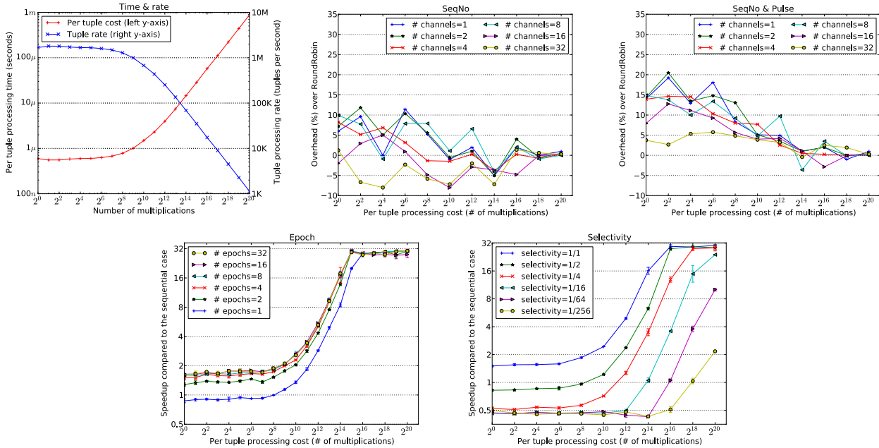
Figure 8: Microbenchmarks.
