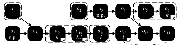
Figure 5: Parallel region formation example. Operator instances labeled “n.p.” are not parallelizable, for example, due to unknown state or selectivity > 1 . The letters k and l indicate key attributes. The dotted line from o_{12} to o_{14} indicates a fusion dependency. Dashed ovals indicate unexpanded parallel regions as in Figure 2. The paper icons in the lower right of an operator indicate the operator is stateful.
