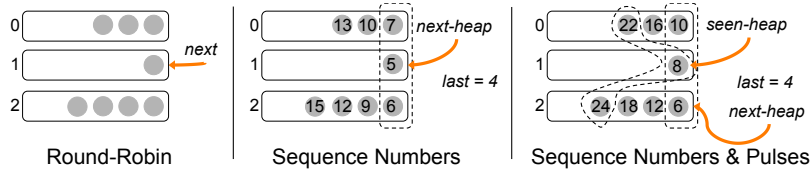
Figure 4: Merge ordering mechanisms after receiving a new tuple.
