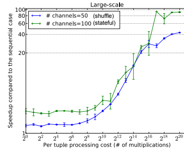
Figure 10: Large-scale scalability.
