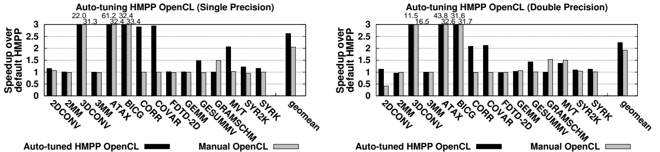
Figure 9: Speedup of auto-tuned HMPP-generated OpenCL kernels and hand-written OpenCL codes over default HMPP OpenCL on 2D/3D convolution and PolyBench codes using single and double precision.
