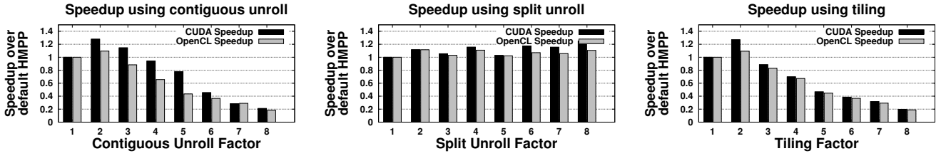
Figure 5: Speedup in 2D CONV using (from left to right) ‘contiguous’ unrolling, ‘split’ unrolling, and tiling with factors 1-8 in the inner loop. The loops are in the initial order and outer loop is not unrolled.
