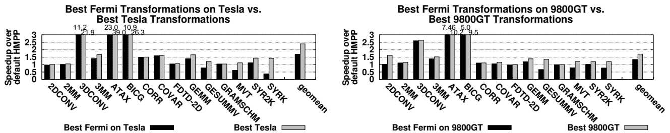
Figure 10: Left: Results of running best CUDA HMPP transformations found on C2050 (Fermi) on GTX 280 (Tesla) vs. best configurations found using auto-tuning on GTX 280 (Tesla); Right: Results of running best CUDA HMPP transformations found on C2050 (Fermi) on 9800 GT vs. best configurations found using auto-tuning on 9800 GT.
