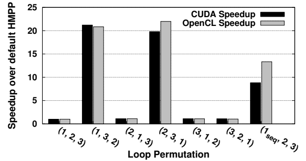
Figure 7: Speedup over default HMPP in 3D CONV using different permutations with default parallelization and initial permutation with 2nd and 3rd loops parallelized.
