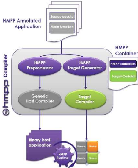
Figure 2: HMPP framework used for turning a sequential C program with specific pragmas to an optimized GPU program. (graphic courtesy of CAPS Enterprise)
