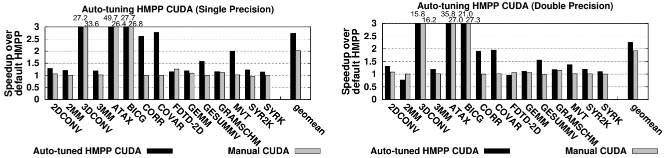
Figure 8: Speedup of auto-tuned HMPP-generated CUDA kernels and hand-written CUDA codes over default HMPP CUDA on 2D/3D convolution and PolyBench codes using single and double precision.
