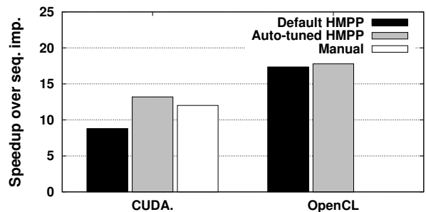
Figure 12: Speedup over sequential implementation of default and optimized HMPP belief propagation on CUDA and OpenCL and of manual implementation on CUDA.
