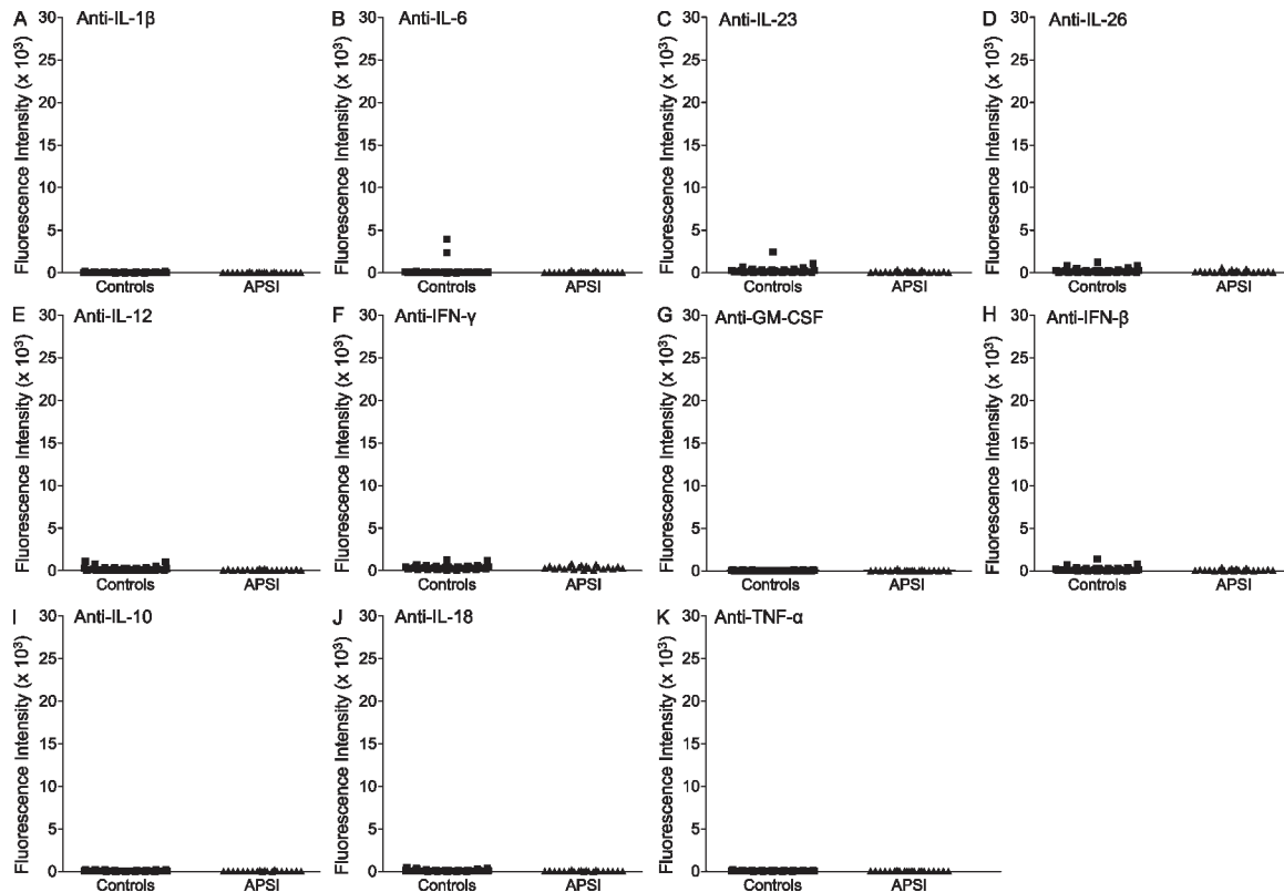
Figure S3. No auto-Abs against IL-1 \beta , IL-6, IL-23, IL-26, IL-12, IFN- \gamma , GM-CSF, IFN- \beta , IL-10, IL-18, and TNF in the plasma from patients with APS-I. (A-K) Anti-IL-1 \beta , -IL-6, -IL-23, -IL-26, -IL-12, -IFN- \gamma , -GM-CSF, -IFN- \beta , -IL-10, -IL-18, and -TNF circulating IgG titers measured by multiplex particle-based flow cytometry in 37 samples from healthy controls and 33 samples from patients with APS-I. FI is plotted on the y axis.
