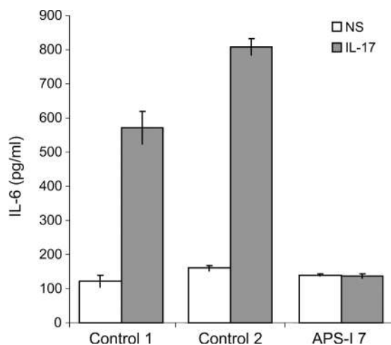
Figure 3. Neutralizing auto-Abs against IL-17A in the plasma from a patient with APS-I. IL-6 production, after 48 h of stimulation with 50 ng/ml IL-17A, by control SV-40-transformed fibroblasts incubated with 10% plasma from two controls or from one patient (APS-I patient 7; means and errors bars from duplicates are shown). The data shown are representative of two experiments.
