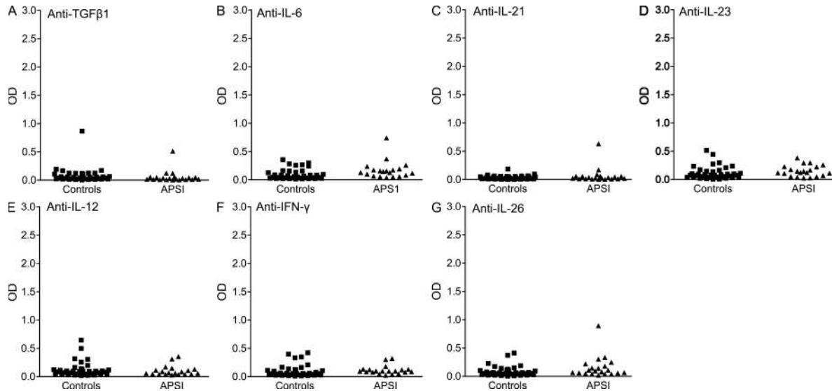
Figure S2. No auto-Abs against TGF-β1, IL-6, IL-21, IL-23, IL-12, IFN-γ, and IL-26 in the plasma from patients with APS-I. (A–G) Anti-TGF-β1, -IL-6, -IL-21, -IL-23, -IL-12, -IFN-γ, and -IL-26 circulating IgG titers were measured by classical ELISA in 37 samples from healthy controls and 30 samples from patients with APS-I. OD 450–630 is plotted on the y axis.
