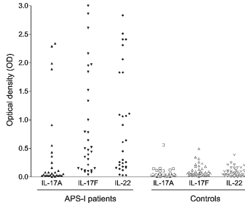
Figure S1. High titers of auto-Abs against IL-17A, IL-17F, and IL-22 in the plasma from patients with APS-I. Anti-IL-17A, -IL-17F, and -IL-22 circulating IgG titers were measured by classical ELISA on 30 samples from patients with APS-I and 37 samples from healthy controls. OD 450–630 is plotted on the y axis. The data shown are representative of two experiments.
