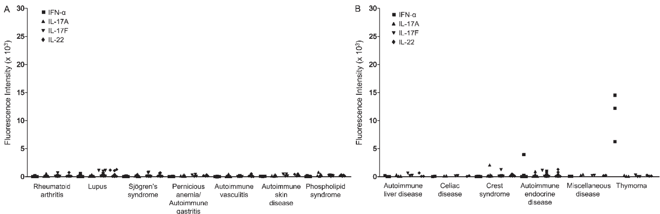
Figure S4. No auto-Abs against IL-17A, IL-17F, and IL-22 in the plasma from patients with autoimmune and/or endocrine disorders. (A and B) Anti-IFN- \alpha , -IL-17A, -IL-17F, and -IL-22 antibodies were measured in 103 patients suffering from autoimmune and/or endocrine disorders: rheumatoid arthritis ( n = 12 ), lupus ( n = 17 ), Sjögren's syndrome ( n = 8 ), pernicious anemia/autoimmune gastritis ( n = 4 ), autoimmune vasculitis ( n = 10 ), autoimmune skin diseases ( n = 4 ), phospholipid syndrome ( n = 5 ), autoimmune liver disease ( n = 3 ), celiac disease ( n = 2 ), CREST syndrome ( n = 7 ), autoimmune endocrine diseases (hypothyroidism, n = 14 ; Graves' disease, n = 6 ; type 1 diabetes, n = 6 ), miscellaneous diseases ( n = 2 ), and thymoma ( n = 3 ).
